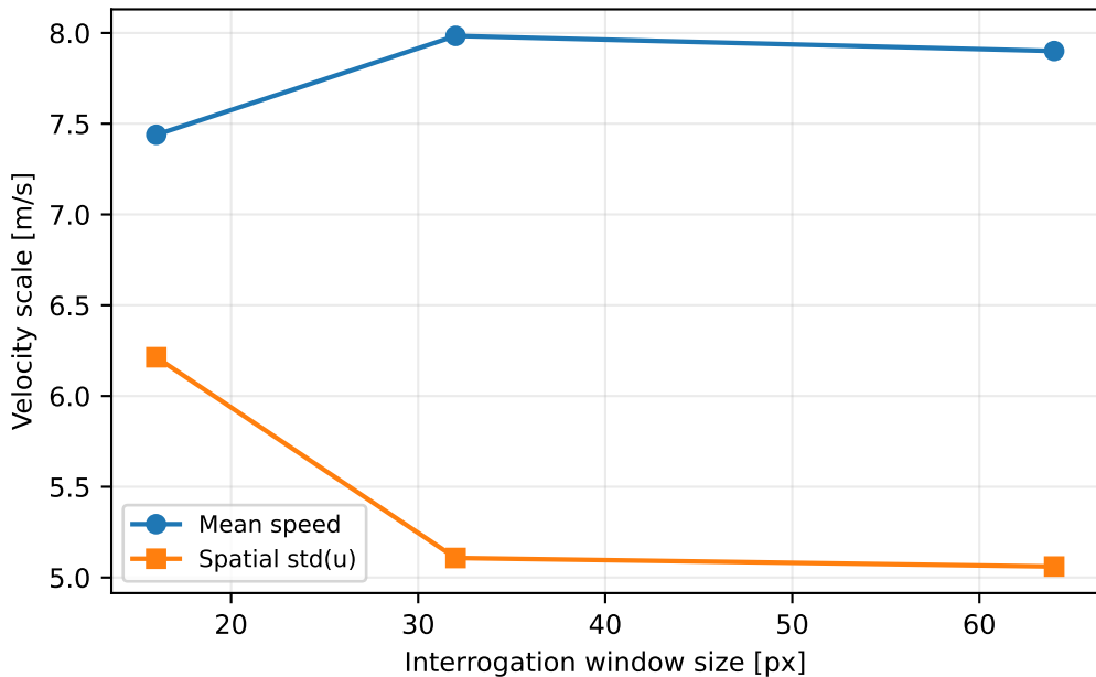
Self-made PIV window-size sensitivity
