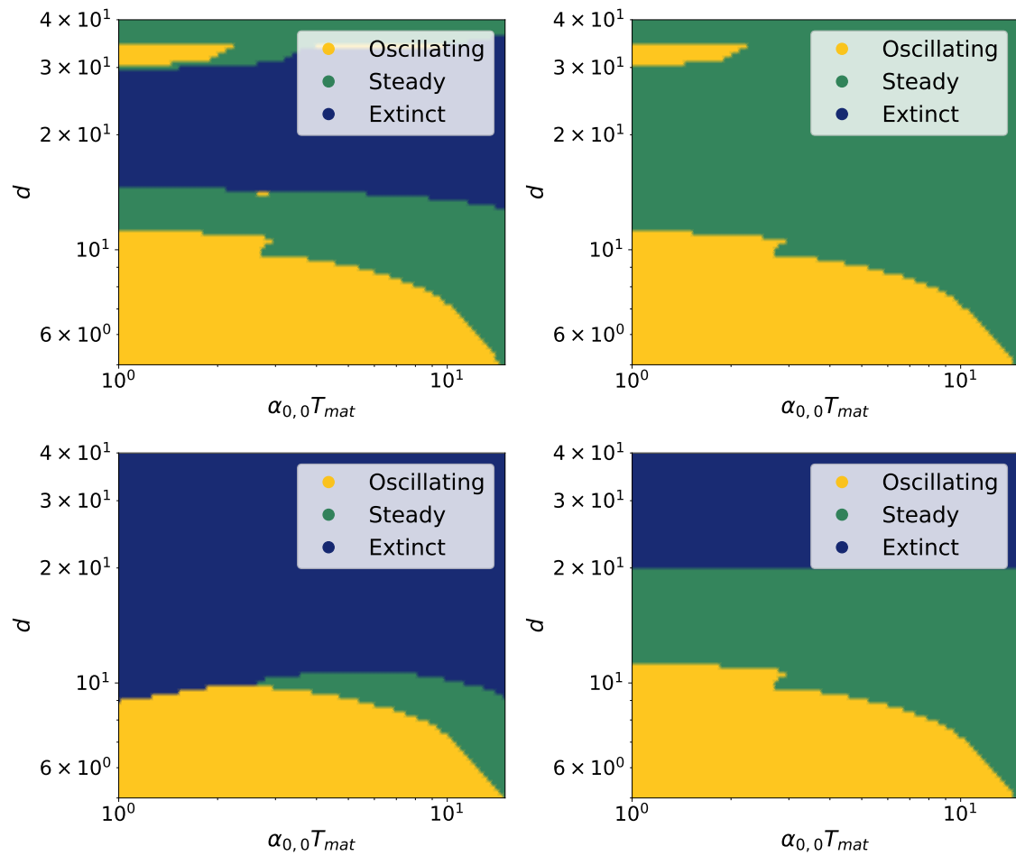
Figure 20: Coexistence diagram of the states of the system in model A (theoretical expectations) after 300 cycles. We used for replication rates \alpha_{0,0} = 5 \times 10^{-1} h^{-1} , \alpha_{1,1} = 2 h^{-1} , \gamma_{0,0} = 7 h^{-1} , \gamma_{1,1} = 20 h^{-1} , and for mutation rates \mu_0 = 7 \times 10^{-3} h^{-1} , \nu_0 = 7 \times 10^{-3} h^{-1} . The carrying capacities are K_p = K_r = 30 and dilution factor d = 10 . The panels represent the fractions for x_0, x_1, z_0, z_1 from right to left and from top to bottom.
