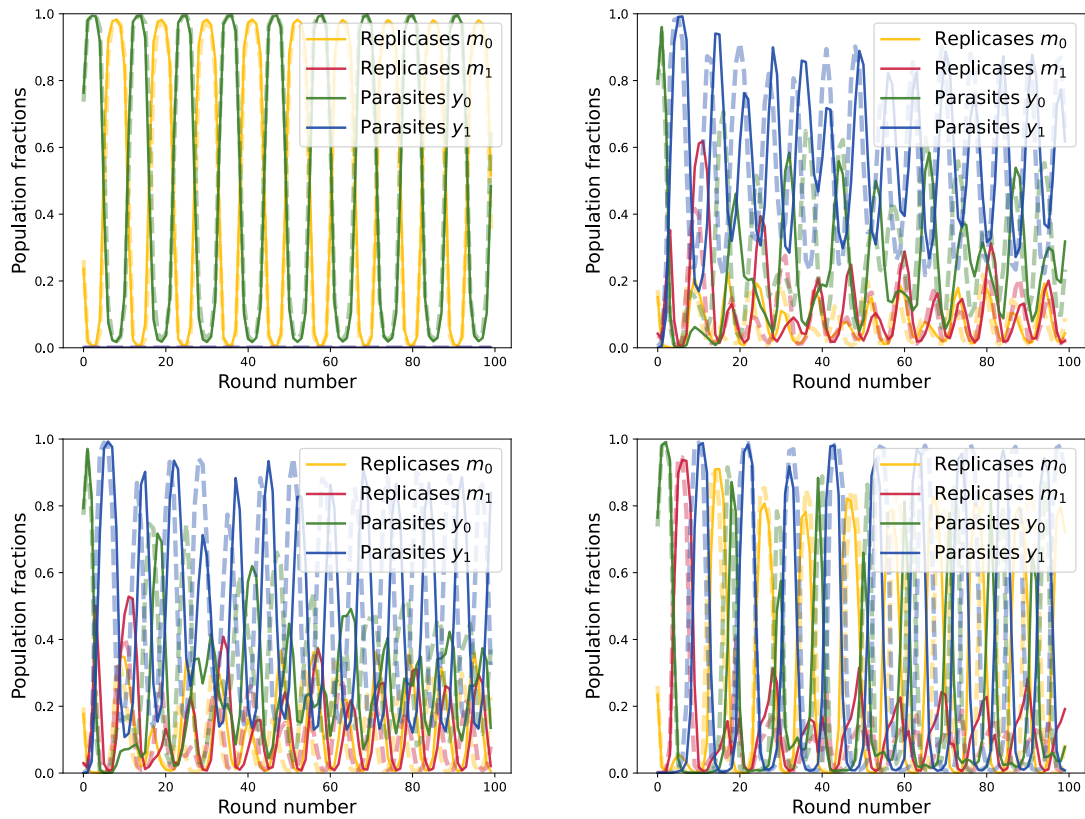
Figure 37: Dynamics with different carrying capacities for parasites and replicases within model B. We used for replication rates \alpha_{0,0} = 5 \times 10^{-1} h^{-1} , \alpha_{1,1} = 2 h^{-1} , \gamma_{0,0} = 7 h^{-1} , \gamma_{1,1} = 20 h^{-1} . Upper left \mu = \nu = 0 h^{-1} . Upper right \mu = \nu = 10^{-2} h^{-1} . Lower left \mu = \nu = 7.10^{-3} h^{-1} . Lower right \mu = \nu = 2.10^4 h^{-1} .
