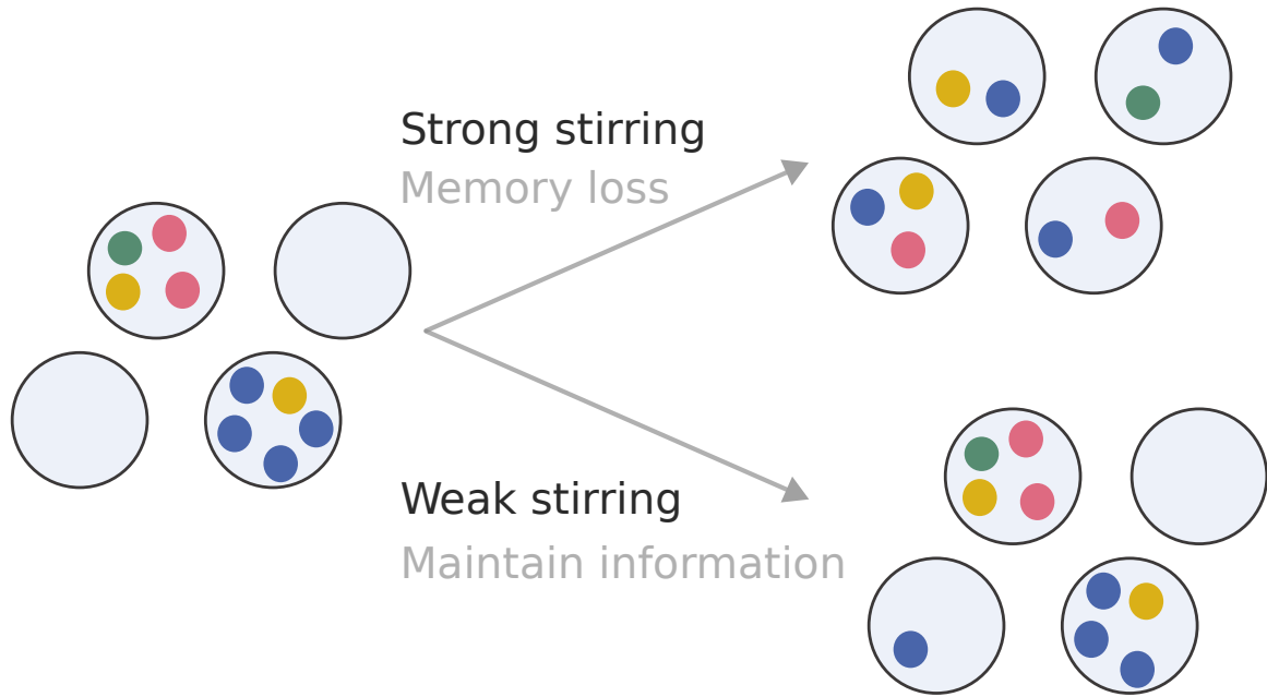
Figure 12: Memory for stirring. With strong stirring, the compartments are homogenized and partially erase their compositional memories. With weak stirring, compartments inherit from their former content after each stirring step and retain some compositional memory.
