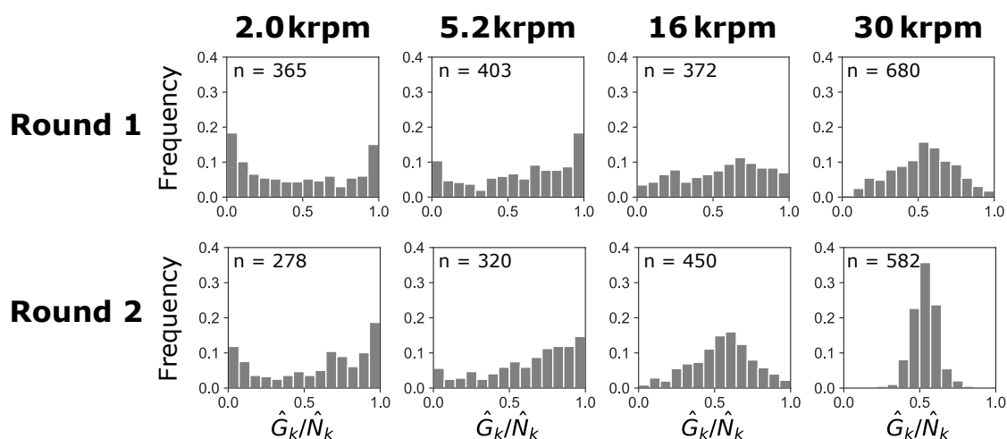
Figure 17: Distribution of fluorescent intensities over two rounds of the transfer experiment. The ratio of FITC fluorescence \hat{G}_k/\hat{N}_k for each droplet containing FITC- or TRITC-labeled dextran was obtained by image analysis. Data for each condition were collected from three independent experiments. The number of analyzed droplets is indicated in each panel.
