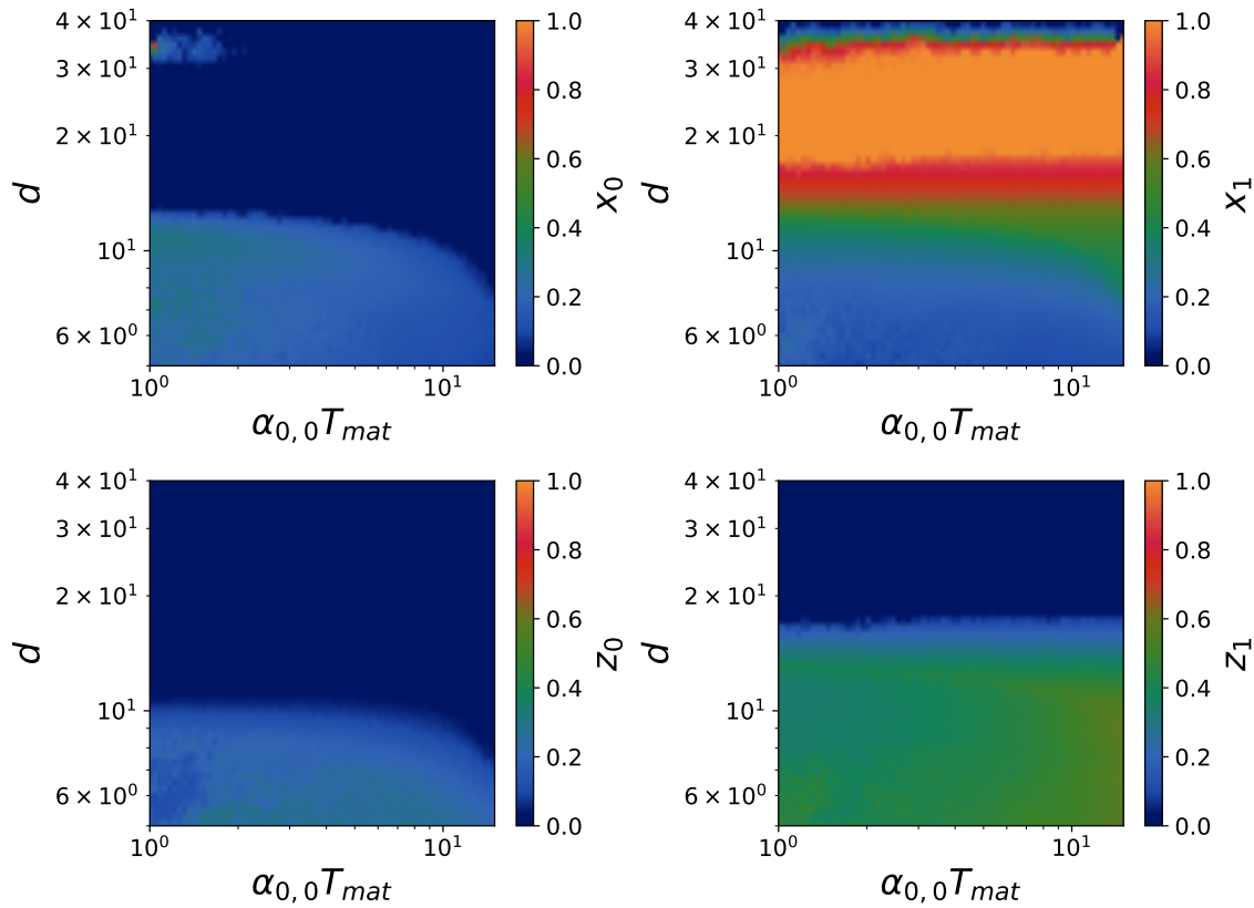
Figure 25: Coexistence diagram with s = 0.95 for the fractions in model A with stirring after 100 cycles with 8000 compartments. We used for replication rates \alpha_{0,0} = 5 \times 10^{-1} h^{-1} , \alpha_{1,1} = 2 h^{-1} , \gamma_{0,0} = 7 h^{-1} , \gamma_{1,1} = 20 h^{-1} , and for mutation rates \mu_0 = 7 \times 10^{-3} h^{-1} , \nu_0 = 7 \times 10^{-3} h^{-1} . The carrying capacities are K_p = K_r = 30 and dilution factor d = 10 . The panels represent the fractions for x_0, x_1, z_0, z_1 from right to left and from top to bottom.
