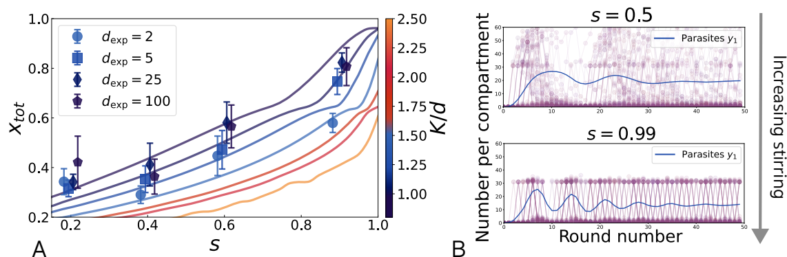
Figure 3: A Total fraction of replicases in the system, x_{tot} . Theoretical expectations (solid lines) are shown for different values of the ratio of carrying capacity to dilution factor K/d . Experimental data (solid symbols) are plotted against stirring strength (2.0, 5.2, 16, and 30 krpm), converted into the corresponding stirring parameters s . For visualization, the data points are plotted at the expected s \pm 0.01 \pm 0.02 . The experiments were performed at different dilution factors, d_{exp} , as indicated in the panel. The same trends are observed in theory and experiments. Error bars indicate the mean \pm one standard deviation ( n = 3-4 ). B Effect of stirring on the compartment composition. In purple, we show the trajectories of individual compartments (for the number of mutant parasites y_1 ), while in solid blue lines we show the average over all compartments. As stirring gets stronger, the contents of compartments homogenize, and the compartments end up either full of mutant parasites or containing mostly no mutant parasites. In this limit, all compositional memory is lost.
