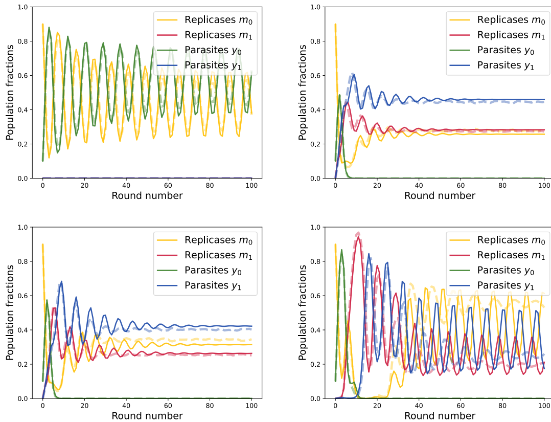
Figure 8: Theoretical prediction for model A (full) of the evolution of the system compared to Gillespie simulations (dotted) performed with 50000 compartments. We used for replication rates \alpha_{0,0} = 5 \times 10^{-1} \text{ h}^{-1} , \alpha_{1,1} = 2 \text{ h}^{-1} , \gamma_{0,0} = 7 \text{ h}^{-1} , \gamma_{1,1} = 20 \text{ h}^{-1} . The carrying capacities are K_p = K_r = 30 and dilution factor d = 10 . The different panels correspond to different mutation rates. Upper left \mu = \nu = 0 \text{ h}^{-1} . Upper right \mu = \nu = 10^{-2} \text{ h}^{-1} . Lower left \mu = \nu = 7.10^{-3} \text{ h}^{-1} . Lower right \mu = \nu = 2.10^4 \text{ h}^{-1} .
