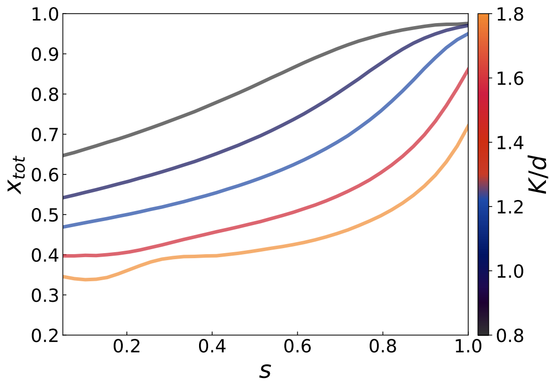
Figure 13: Total fraction of replicases x_{tot} depending on the stirring parameter s with two species (one replicase and one parasite). The colour bar indicates the value of the ratio carrying capacity to dilution K/d . The lower it is, the less compartments should be populated.
