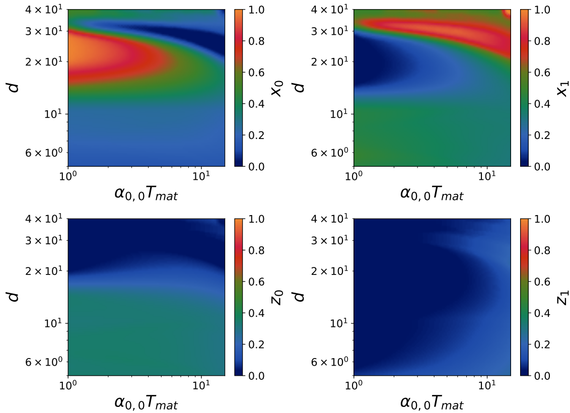
Figure 31: Coexistence diagram of the fractions of each species in the system with the improvement of resistance in model B (theoretical expectations) after 300 cycles. We used for replication rates \alpha_{0,0} = 5 \times 10^{-1} h^{-1} , \alpha_{1,1} = 5 \times 10^{-1} h^{-1} , \gamma_{0,0} = 10 h^{-1} , \gamma_{1,1} = 5 \times 10^{-1} h^{-1} , and for mutation rates \mu_0 = 7 \times 10^{-3} h^{-1} , \nu_0 = 7 \times 10^{-3} h^{-1} . The carrying capacities are K_p = K_r = 30 and dilution factor d = 10 . The panels represent the fractions for x_0, x_1, z_0, z_1 from right to left and from top to bottom.
