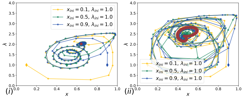
Figure 11: Oscillations between \lambda and x_{tot} with four species and within model B. The initial conditions are shown with diamonds. In red we represent the typical oscillation pattern towards which the system equilibrate, if K/d is large enough. For smaller K/d the system reaches a steady state. (i) K = 29, d = 10 , (ii) K = 32, d = 10 .
