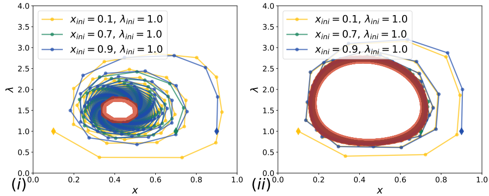
Figure 10: Oscillations between \lambda and x_{tot} with two species. The initial conditions are shown with diamonds. In red we represent the typical oscillation pattern towards which the system equilibrate, if K/d is large enough. For smaller K/d the system reaches a steady state. (i) K = 29, d = 10 , (ii) K = 32, d = 10 .
