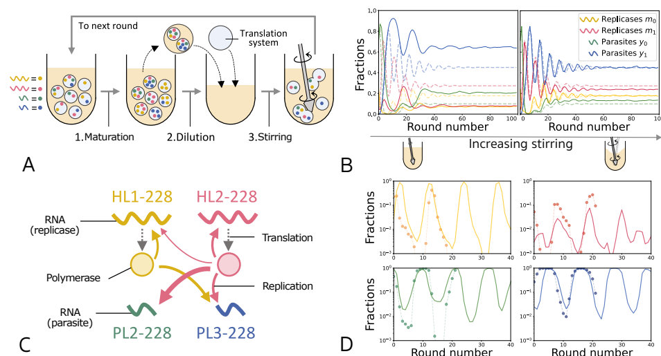
Figure 2: A Schematic representation of the long-term replication experiment. 1) RNAs were replicated in water-in-oil droplets at 37^{\circ}\text{C} for 5 h. 2) Droplets were five-fold diluted with a fresh oil phase and the translation system. 3) The droplet population was stirred, allowing fusion and division, thereby redistributing RNAs among droplets. B Effect of stirring on the dynamics, we used the same deterministic rules and parameters but for different values of the stirring parameter s ( s=0.5 and s=0.99 ). The solid lines represent the simulations with stirring while the dotted lines represent the perfectly homogeneous case. Simulations with stirring were performed with 50000 compartments, the carrying capacities are K_p = K_r = 30 and dilution factor d = 10 . Oscillations are damped in this panel because K/d is small enough, (as illustrated in Fig. 1D and detailed in SI appendix Section 1.F). C The RNA replication system containing two replicases (HL1-228 in yellow and HL2-228 in red) and two parasites (PL2-228 in green and PL3-228 in blue). These RNAs replicate by utilizing polymerases translated from the replicases. The widths of the colored arrows represent relative replication efficiencies [37]. D We can reproduce experimental dynamics of four RNA species (2 replicases and 2 parasites), represented by solid circles connected by thin dashed lines. The solid lines show simulations performed using the same dilution factor d = 5 and the experimentally determined replication rates of the individual species [34]. Each species has a different carrying capacity, determined by its length. Other parameters are detailed in SI appendix Section 2.D.
