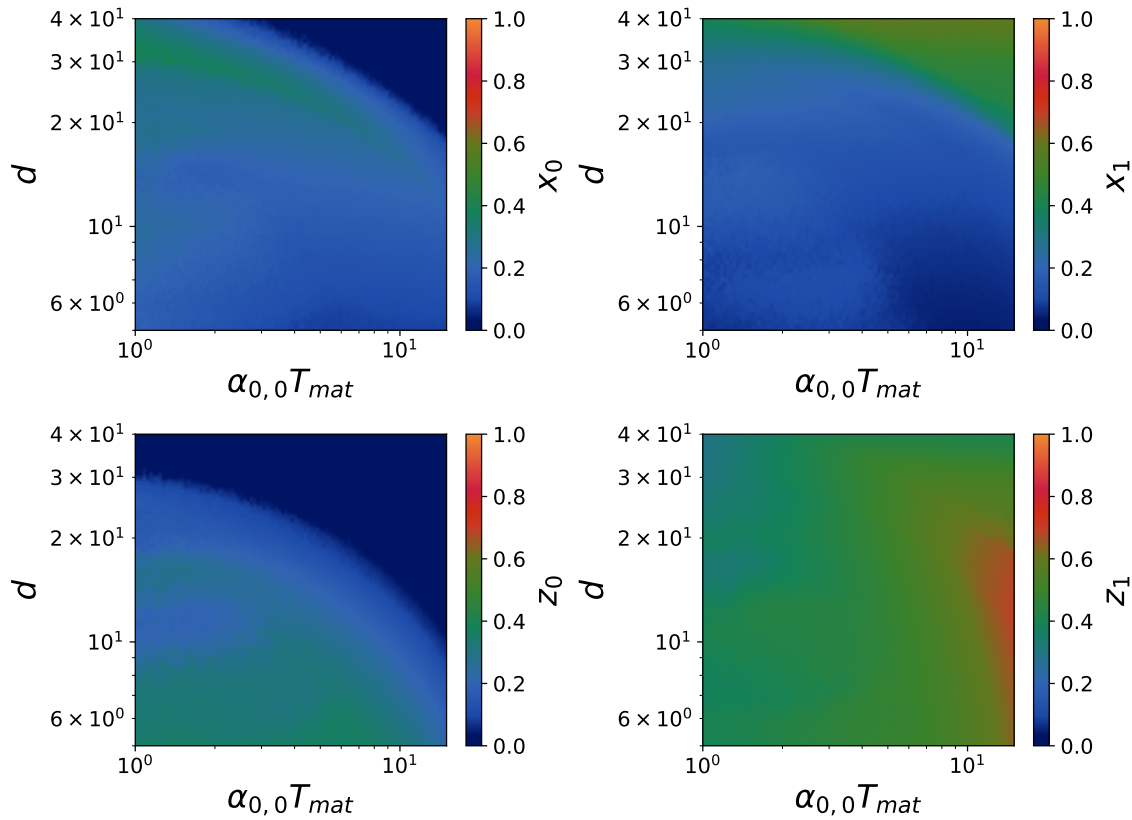
Figure 24: Coexistence diagram with s = 0.7 for the fractions in model A with stirring after 100 cycles with 8000 compartments. We used for replication rates \alpha_{0,0} = 5 \times 10^{-1} h^{-1} , \alpha_{1,1} = 2 h^{-1} , \gamma_{0,0} = 7 h^{-1} , \gamma_{1,1} = 20 h^{-1} , and for mutation rates \mu_0 = 7 \times 10^{-3} h^{-1} , \nu_0 = 7 \times 10^{-3} h^{-1} . The carrying capacities are K_p = K_r = 30 and dilution factor d = 10 . The panels represent the fractions for x_0, x_1, z_0, z_1 from right to left and from top to bottom.
