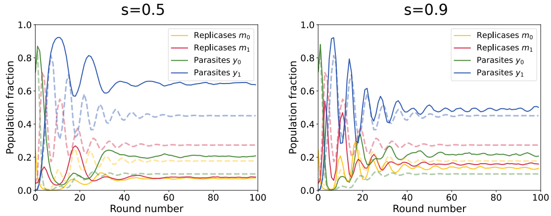
Figure 28: Illustration of the discrepancy between s = 1 and imperfect stirring with model B for \alpha_{0,0} = 5 \times 10^{-1} h^{-1} , \alpha_{1,1} = 2 h^{-1} , \gamma_{0,0} = 7 h^{-1} , \gamma_{1,1} = 20 h^{-1} , and \mu_0, \nu_0 = \nu_1 = 7 \times 10^{-3} h^{-1} and 50000 compartments. The carrying capacities are K_p = K_r = 30 and dilution factor d = 10 . The panels represent different values of the stirring parameter s .
