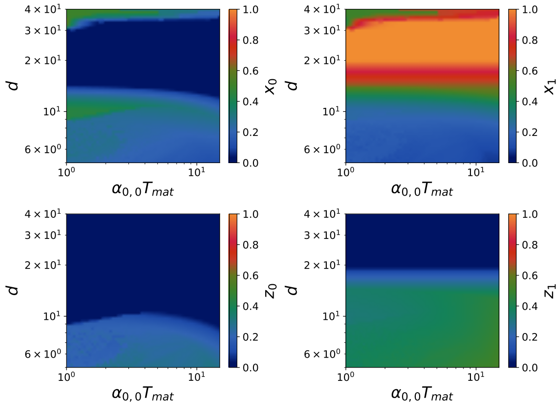
Figure 29: Coexistence diagram for the fractions in model A with generalist parasites (theoretical expectations) after 300 cycles. We used for replication rates \alpha_{0,0} = 5 \times 10^{-1} h^{-1} , \alpha_{1,1} = 2 h^{-1} , \gamma_{0,0} = 7 h^{-1} , \gamma_{1,1} = 20 h^{-1} , and for mutation rates \mu_0 = 7 \times 10^{-3} h^{-1} , \nu_0 = 7 \times 10^{-3} h^{-1} . The carrying capacities are K_p = K_r = 30 and dilution factor d = 10 . The panels represent the fractions for x_0, x_1, z_0, z_1 from right to left and from top to bottom.
