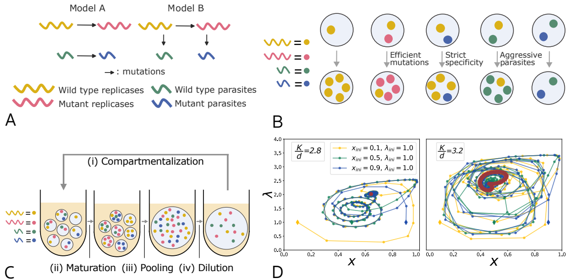
Figure 1: A Representation of two possible evolution models of the RNA replication system containing two replicases and two parasites. B Illustration of the deterministic assumptions. C Transient compartmentalization with pooling (homogeneous case). D Illustration of the typical oscillatory dynamics obtained with the deterministic approach with second order replication rates and mutations. Here we show the results for model B, we used the rates \alpha_{0,0} = 0.5h^{-1} , \alpha_{1,1} = 2.0h^{-1} , \gamma_{0,0} = 7.0h^{-1} , \gamma_{1,1} = 20.0h^{-1} , \mu_0 = 1.0 \times 10^{-2}h^{-1} , \nu_0 = 1.0 \times 10^{-2}h^{-1} and \nu_1 = 1.0 \times 10^{-2}h^{-1} . The carrying capacities are K = K_r = K_p = 28 on the left panel and K = K_r = K_p = 32 on the right panel, and the dilution factor is d = 10 . Limit cycles are shown in red (which is a single point for a steady state). We observe damped oscillations reaching a steady state on the left panel, and sustained oscillations (limit cycles) on the right panel.
