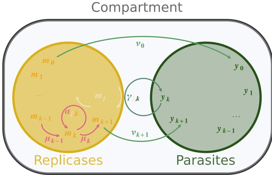
Figure 6: Processes occurring during maturation (model B). Replicases of type 0, 1, \dots, k+1 are shown on the left (yellow disk) and parasites of type 0, 1, \dots, k+1 on the right (green disk). Replicase k can be replicated by replicase j at a rate \alpha_{j,k} , and mutate to replicase k+1 at a rate \mu_k , and to parasite of type k at a rate \nu_k . Parasite k can be replicated by replicase j at a rate \gamma_{j,k} .
