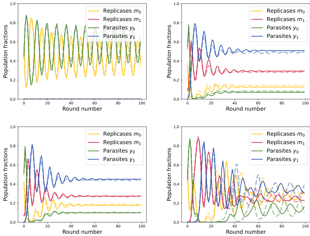
Figure 9: Theoretical prediction for model B (full) of the evolution of the system compared to Gillespie simulations (dotted) performed with 50000 compartments. We used for replication rates \alpha_{0,0} = 5 \times 10^{-1} \text{ h}^{-1} , \alpha_{1,1} = 2 \text{ h}^{-1} , \gamma_{0,0} = 7 \text{ h}^{-1} , \gamma_{1,1} = 20 \text{ h}^{-1} . The carrying capacities are K_p = K_r = 30 and dilution factor d = 10 . The different panels correspond to different mutation rates. Upper left \mu = \nu = 0 \text{ h}^{-1} . Upper right \mu = \nu = 10^{-2} \text{ h}^{-1} . Lower left \mu = \nu = 7.10^{-3} \text{ h}^{-1} . Lower right \mu = \nu = 2.10^4 \text{ h}^{-1} .
