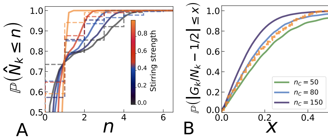
Figure 14: A Experimental distributions of \hat{N}_k (total fluorescence rescaled by the average total fluorescence per compartment) and theoretical predictions. We conclude that taking packets of molecules corresponding to the average total fluorescence per compartment seems to describe well the exchanges between compartments. In dotted lines we show the experimental cumulative probability distributions (discretized because it represents the number of packets of molecules emitting a fluorescence equal to the average total fluorescence per compartment). In solid lines we show expectations from the theory. B Comparison of the experimental distribution with maximal stirring (30 krpm) and theory starting from a perfectly bimodal distribution for s \rightarrow 1 , used to calibrate the value n_C = 80 .
