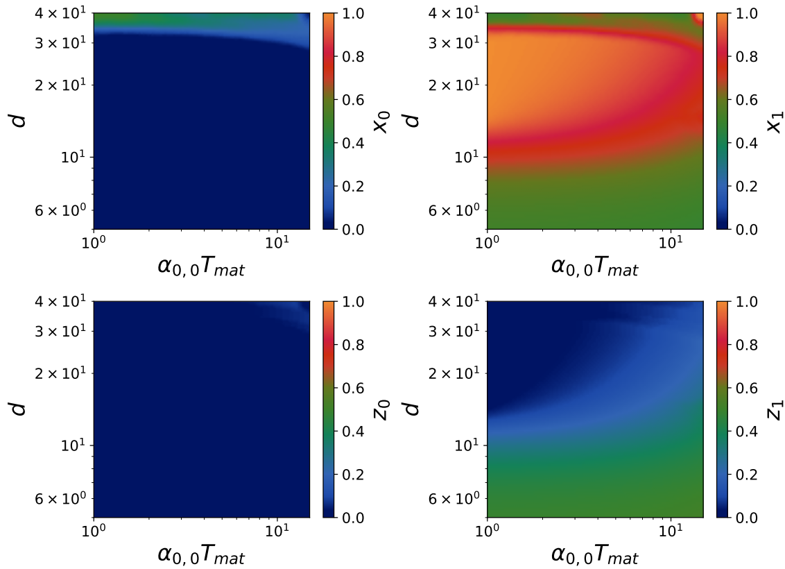
Figure 32: Coexistence diagram of the fractions of each species in the system with a General-ity/Replicability trade-off in model B (theoretical expectations) after 300 cycles. We used for repli-cation rates \alpha_{0,0} = 5 \times 10^{-2} h^{-1} , \alpha_{1,1} = 5 \times 10^{-2} h^{-1} , \gamma_{0,0} = 1. h^{-1} , \gamma_{0,1} = 1 \times 10^{-1} h^{-1} , \gamma_{1,1} = 2.5 \times 10^{-1} h^{-1} , and for mutation rates \mu_0 = 5 \times 10^{-4} h^{-1} , \nu_0 = 5 \times 10^{-4} h^{-1} . The carrying capacities are K_p = K_r = 30 and dilution factor d = 10 . The panels represent the fractions for x_0, x_1, z_0, z_1 from right to left and from top to bottom.
