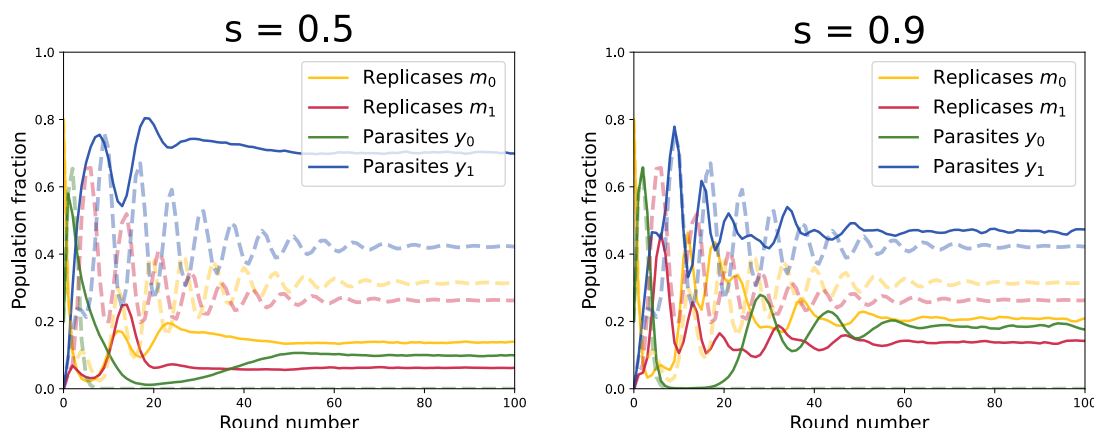
Figure 23: Comparison between complete pooling dynamics and stirring (simulations with stirring were performed with 50000 compartments). In experiments compartments are reinitialized by stirring, we model this in the last section. The stronger is stirring the more the system has a memory. This could explain discrepancies between our model of complete stirring and experiments. We used for replication rates \alpha_{0,0} = 5 \times 10^{-1} h^{-1} , \alpha_{1,1} = 2 h^{-1} , \gamma_{0,0} = 7 h^{-1} , \gamma_{1,1} = 20 h^{-1} , and for mutation rates \mu_0 = 7 \times 10^{-3} h^{-1} , \nu_0 = 7 \times 10^{-3} h^{-1} . The carrying capacities are K_p = K_r = 30 and dilution factor d = 10 . The panels represent different values of the stirring parameter s .
