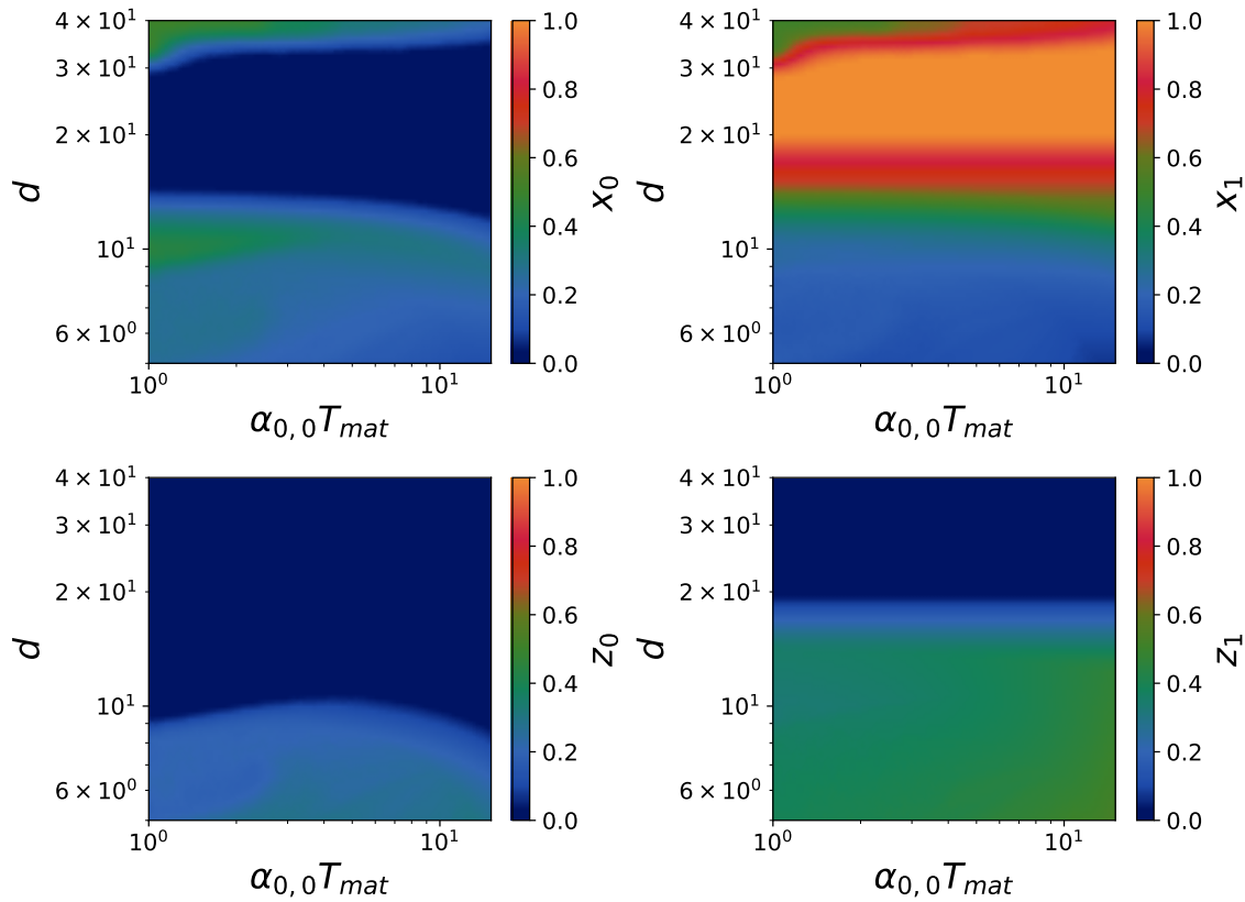
Figure 19: Coexistence diagram for the fractions in model A (theoretical expectations) after 300 cycles. We used for replication rates \alpha_{0,0} = 5 \times 10^{-1} h^{-1} , \alpha_{1,1} = 2 h^{-1} , \gamma_{0,0} = 7 h^{-1} , \gamma_{1,1} = 20 h^{-1} , and for mutation rates \mu_0 = 7 \times 10^{-3} h^{-1} , \nu_0 = 7 \times 10^{-3} h^{-1} . The carrying capacities are K_p = K_r = 30 and dilution factor d = 10 . The panels represent the fractions for x_0, x_1, z_0, z_1 from right to left and from top to bottom.
