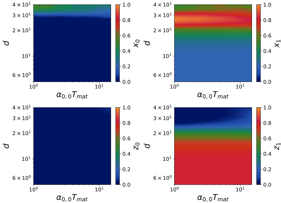
Figure 39: Coexistence diagram of the states of the system in model B in a Generality/Replicability trade-off after 300 cycles. We used for replication rates \alpha_{0,0} = 5 \times 10^{-2} h^{-1} , \alpha_{1,1} = 5 \times 10^{-2} h^{-1} , \gamma_{0,0} = 1. h^{-1} , \gamma_{0,1} = 1 \times 10^{-1} h^{-1} , \gamma_{1,1} = 2.5 \times 10^{-1} h^{-1} , and for mutation rates \mu_0 = 5 \times 10^{-4} h^{-1} , \nu_0 = 5 \times 10^{-4} h^{-1} . The carrying capacities are K_p = 4K_r = 120 and dilution factor d = 10 . The panels represent the fractions for x_0, x_1, z_0, z_1 from right to left and from top to bottom.
