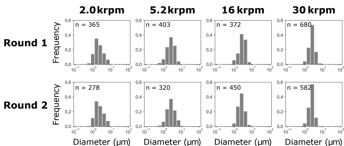
Figure 18: Size distribution of droplets over two rounds of the transfer experiment with fluorescent dyes. The diameters of individual droplets containing FITC- or TRITC-labeled dextran were obtained by image analysis. Data for each condition were collected from three independent experiments. The number of analyzed droplets is indicated in each panel.
