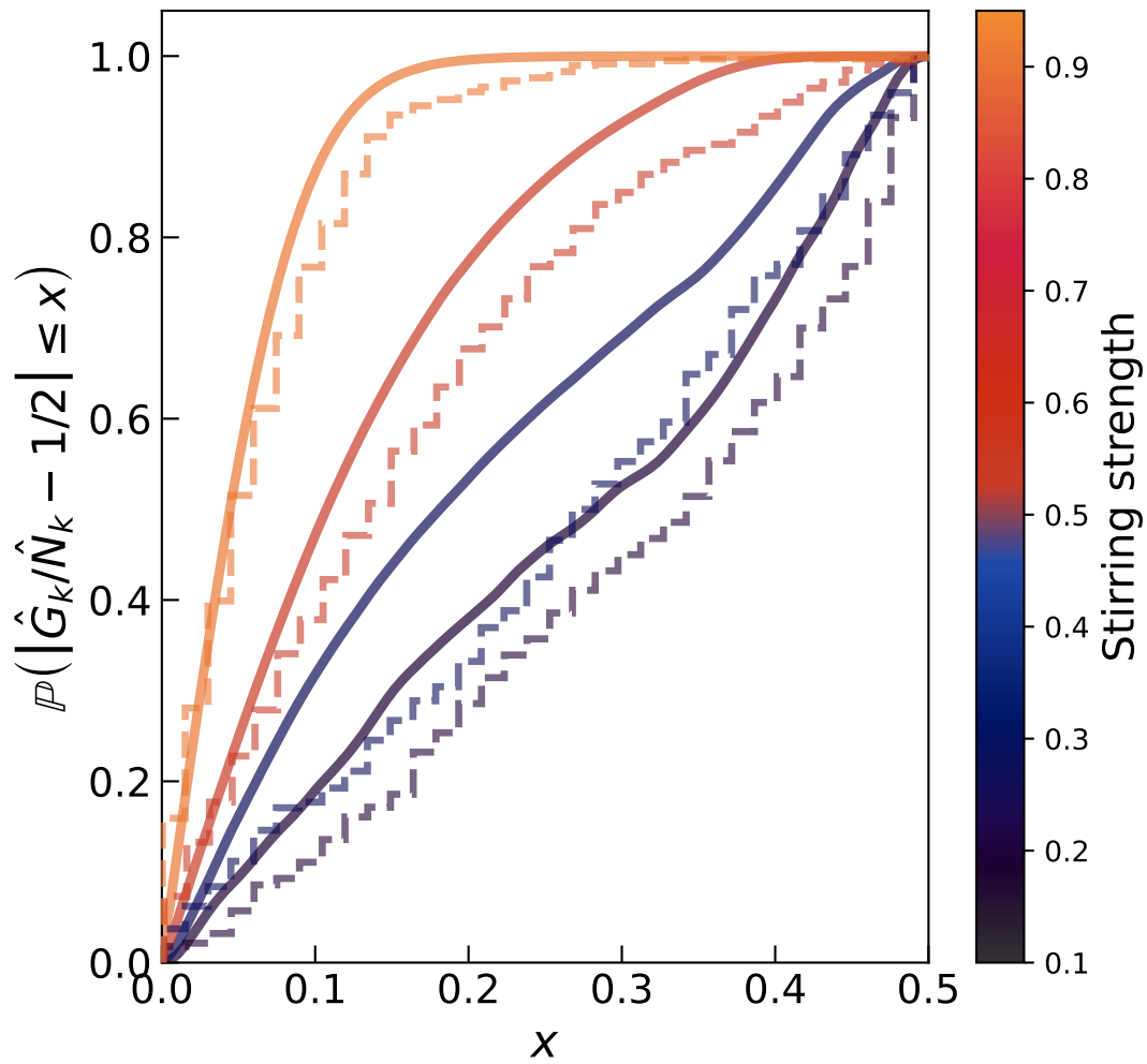
Figure 15: Assessment of the robustness of estimations of s . Starting from experimental distributions before round 2, we apply the theoretical transformation with s inferred from the first round (starting from a perfectly bimodal distribution of \hat{G}_k/\hat{N}_k ) and compare it to the experimental distribution after round 2 for each stirring strengths.
