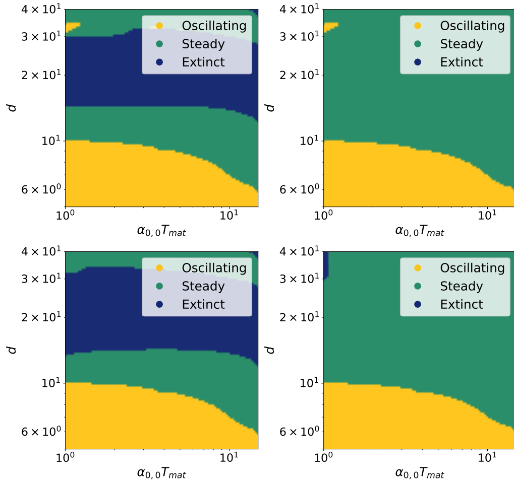
Figure 22: Coexistence diagram of the states of the system in model B where hosts mutate to parasites (theoretical expectations) after 300 cycles. We used for replication rates \alpha_{0,0} = 5 \times 10^{-1} h^{-1} , \alpha_{1,1} = 2 h^{-1} , \gamma_{0,0} = 7 h^{-1} , \gamma_{1,1} = 20 h^{-1} , and for mutation rates \mu_0 = 7 \times 10^{-3} h^{-1} , \nu_0 = 7 \times 10^{-3} h^{-1} , \nu_1 = 7 \times 10^{-3} h^{-1} . The carrying capacities are K_p = K_r = 30 and dilution factor d = 10 . The panels represent the fractions for x_0, x_1, z_0, z_1 from right to left and from top to bottom.
