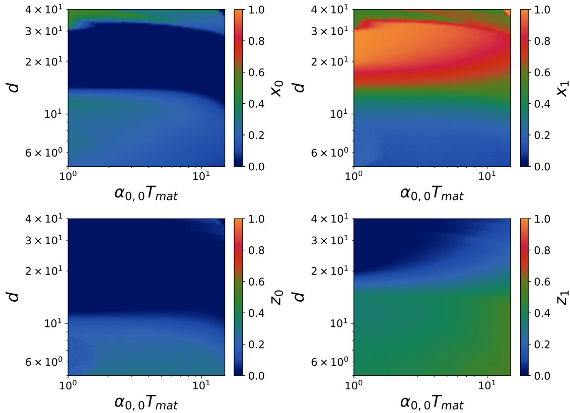
Figure 21: Coexistence diagram for the fractions with model B where hosts mutate to parasites (theoretical expectations) after 300 cycles. We used for replication rates \alpha_{0,0} = 5 \times 10^{-1} h^{-1} , \alpha_{1,1} = 2 h^{-1} , \gamma_{0,0} = 7 h^{-1} , \gamma_{1,1} = 20 h^{-1} , and for mutation rates \mu_0, \nu_0, \nu_1 = 7 \times 10^{-3} h^{-1} . The carrying capacities are K_p = K_r = 30 and dilution factor d = 10 . The panels represent the fractions for x_0, x_1, z_0, z_1 from right to left and from top to bottom.
