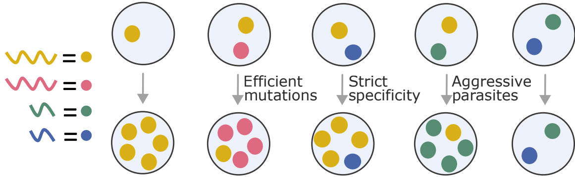
Figure 7: Deterministic approach of the maturation phase. A replicase isolated in a compartment will be able to be replicated freely. In a compartment with different types of replicases, the fittest will take over the compartment, and we assume that fitness increases with mutations ( efficient mutations , otherwise we can switch the roles of mutants and WT to sort them according to their fitness). In a compartment with a replicase and a parasite which is not able to use this replicase, parasites will not be replicated ( strict specificity ). In a compartment with a replicase and parasite able to use this replicase, parasites will take over ( aggressive parasites ). In a compartment with parasites only, parasites will not be replicated.
