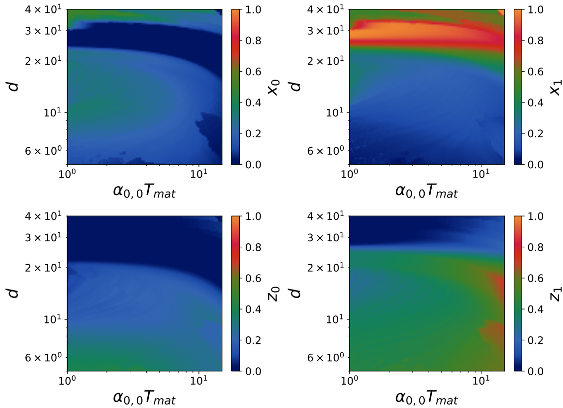
Figure 38: Coexistence diagram of the states of the system in model B where hosts mutate to parasites after 300 cycles. We used for replication rates \alpha_{0,0} = 5 \times 10^{-2} h^{-1} , \alpha_{1,1} = 5 \times 10^{-2} h^{-1} , \gamma_{0,0} = 1. h^{-1} , \gamma_{0,1} = 1 \times 10^{-1} h^{-1} , \gamma_{1,1} = 2.5 \times 10^{-1} h^{-1} , and for mutation rates \mu_0 = 5 \times 10^{-4} h^{-1} , \nu_0 = 5 \times 10^{-4} h^{-1} . The carrying capacities are K_p = 4K_r = 120 and dilution factor d = 10 . The panels represent the fractions for x_0, x_1, z_0, z_1 from right to left and from top to bottom.
