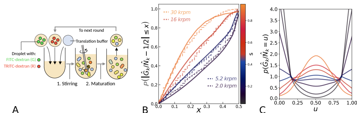
Figure 4: Influence of the stirring parameter s on the distribution of the fraction of one type of individuals, in a population with only two types of individuals. A Experimental procedure to assess the effect of stirring with two fluorescent dyes. After preparing the system from droplets containing either FITC- or TRITC-labeled dextran ( G or R ) together with the translation buffer, as described in the Materials Methods, the system was stirred for 1 min, followed by a 5 h incubation (maturation) phase. B Evolution of the experimental distributions (dotted lines, after round 1) for different stirring strengths and comparison with theoretical distributions (solid lines) starting from a perfectly bimodal distribution of \hat{G}_k/\hat{N}_k for different values of the stirring parameter s . We observe that the distribution of |\hat{G}_k/\hat{N}_k - 1/2| shifts towards 0 as stirring strengths increases, meaning that the distribution of \hat{G}_k/\hat{N}_k shifts towards a monomodal, with a peak close to 0.5. We used n_C = 80 (estimated from data, see SI appendix Section 2) interacting compartments. Experimental stirring was performed for 1 min at four different strengths (2.0, 5.2, 16, 30krpm). For each stirring strength, we evaluated the stirring parameter s yielding a theoretical distribution corresponding the experimental distribution. C Effect of stirring on the probability distribution function of the fraction \hat{G}_k/\hat{N}_k (probability that \hat{G}_k/\hat{N}_k is between u and u + du ) with n_C = 80 interacting compartments, starting from a perfectly bimodal distribution with peaks at \hat{G}_k/\hat{N}_k = 0 and \hat{G}_k/\hat{N}_k = 1 . The distribution shifts towards a monomodal distribution as s increases.
