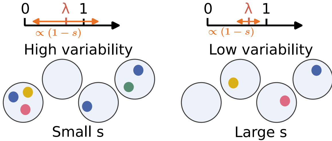
Figure 16: Mechanism for a small number of individuals and high stirring parameter s . When s decreases, the variability of the content of compartments allows for more populated compartments after dilution and stirring, and prevents from extinction. At large values of s , for \lambda \sim 1 , individuals are more likely isolated in one compartment. Isolated parasites cannot replicate, thus this limit typically favours replicases.
