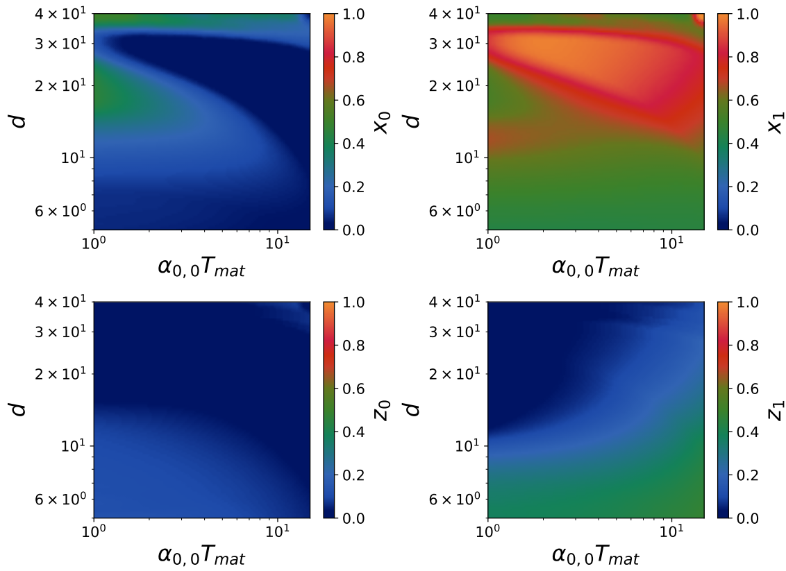
Figure 33: Trade-off Generality/Replicability (slow mutants) with the deterministic approach for s = 1 . We used for replication rates \alpha_{0,0} = 5 \times 10^{-1} h^{-1} , \alpha_{1,1} = 5 \times 10^{-1} h^{-1} , \gamma_{0,0} = 10. h^{-1} , \gamma_{0,1} = 5 \times 10^{-1} h^{-1} , \gamma_{1,1} = 5 \times 10^{-1} h^{-1} , and for mutation rates \mu_0 = 7 \times 10^{-3} h^{-1} , \nu_0 = 7 \times 10^{-3} h^{-1} . The carrying capacities are K_p = K_r = 30 and dilution factor d = 10 .
