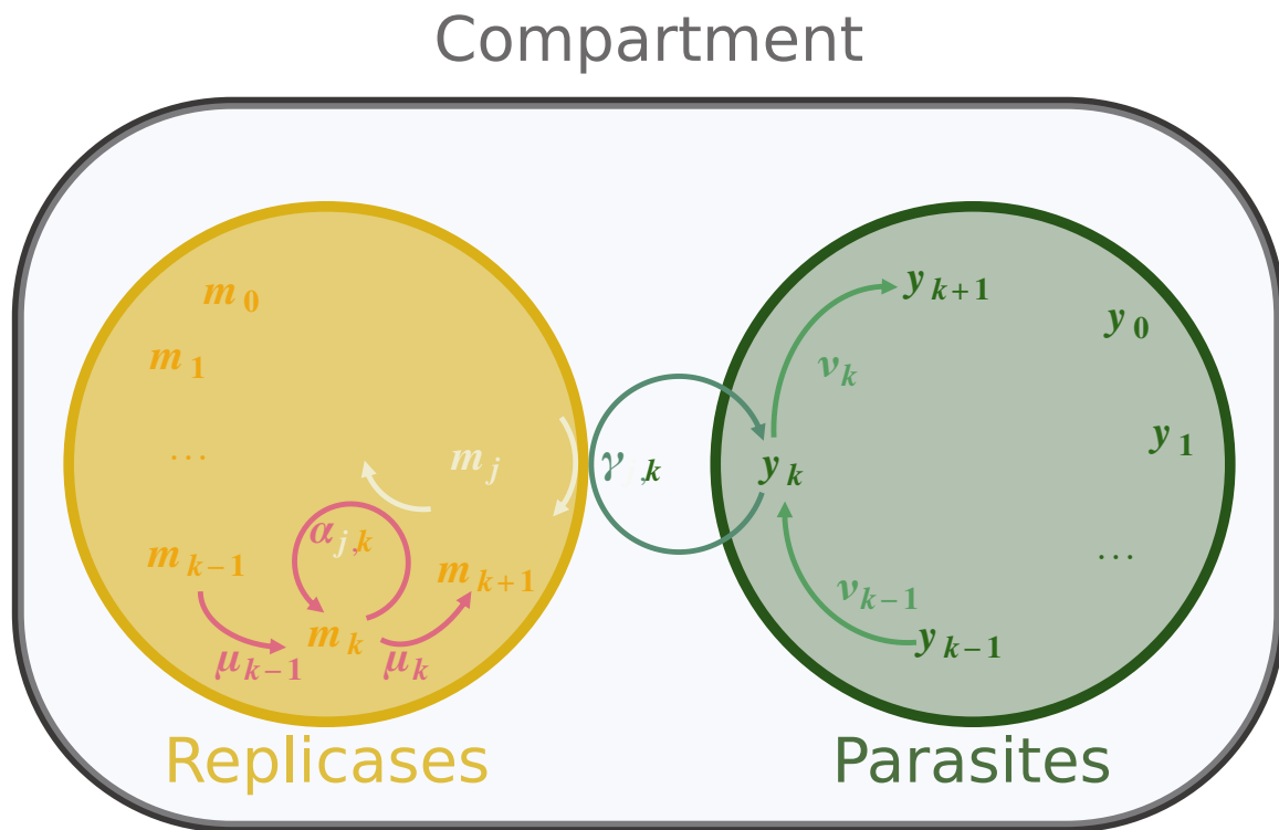
Figure 5: Processes occurring during maturation (model A). Replicases of type 0, 1, \dots, k+1 are shown on the left (yellow disk) and parasites of type 0, 1, \dots, k+1 on the right (green disk). Replicase k can be replicated by replicase j at a rate \alpha_{j,k} , and mutate to replicase k+1 at a rate \mu_k . Parasite k can be replicated by replicase j at a rate \gamma_{j,k} , and mutate to replicase k+1 at a rate \nu_k .
