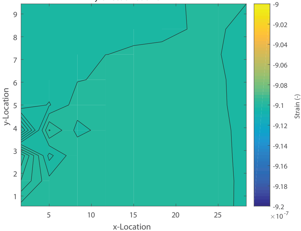
y-direction Strains
