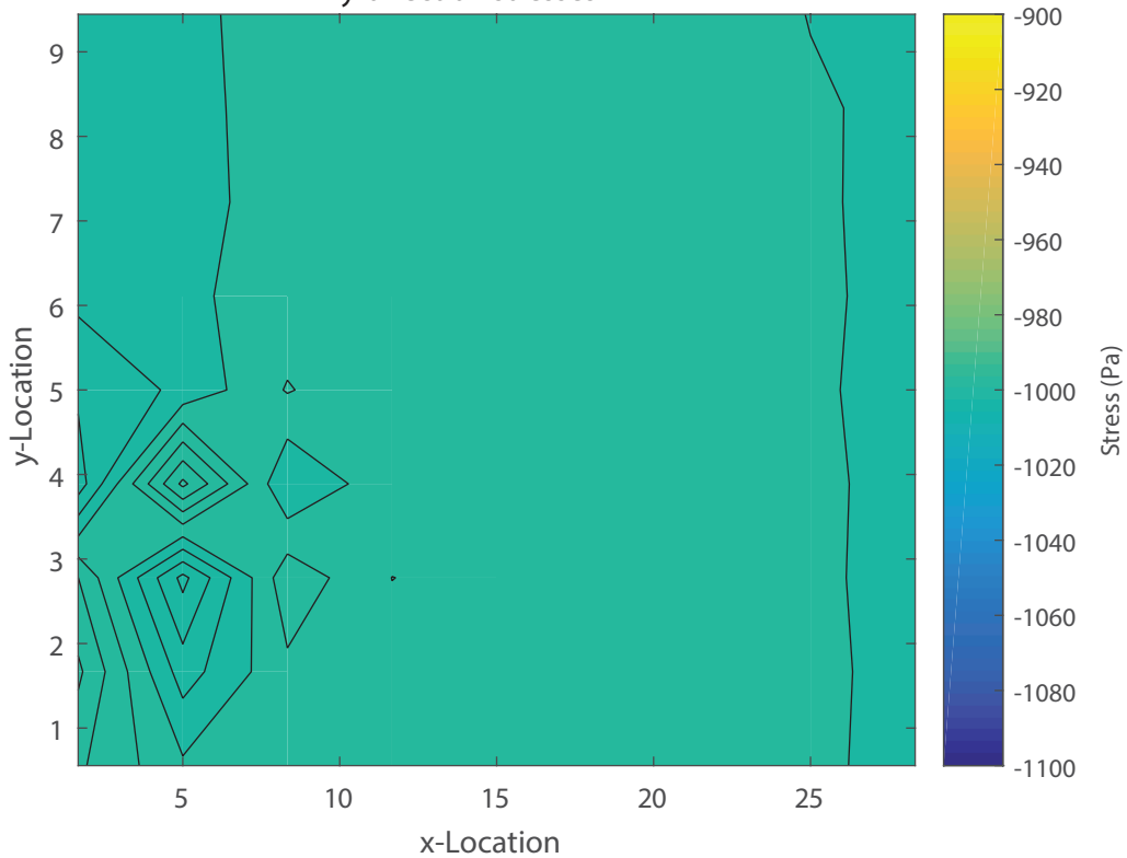
y-direction stresses
