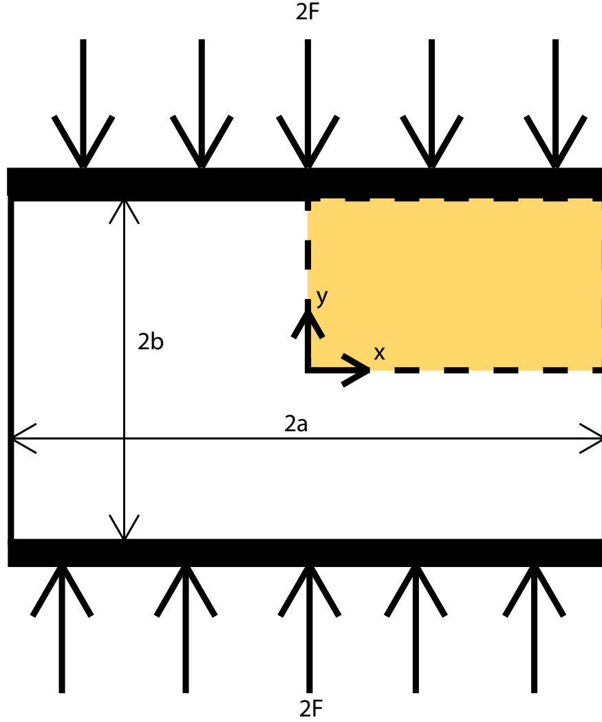
Figure 1: An overview of Mandel's problem.
