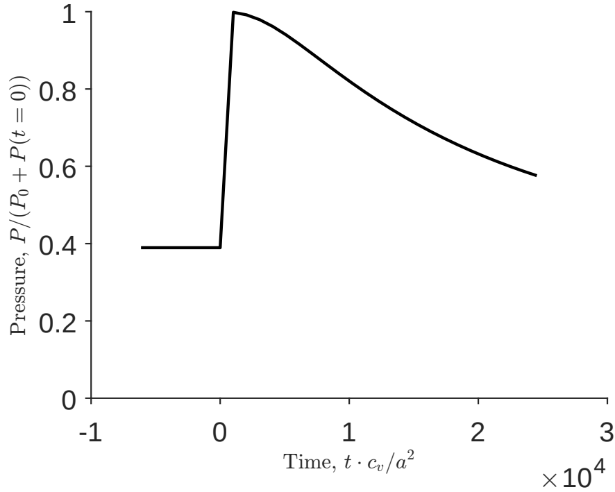
Figure 4: The MATLAB simulator results. Note the Mandel-Cryer effect clearly visible at t = 0 . Additionally the jump in pressure matches the P_0 predicted for this problem.
