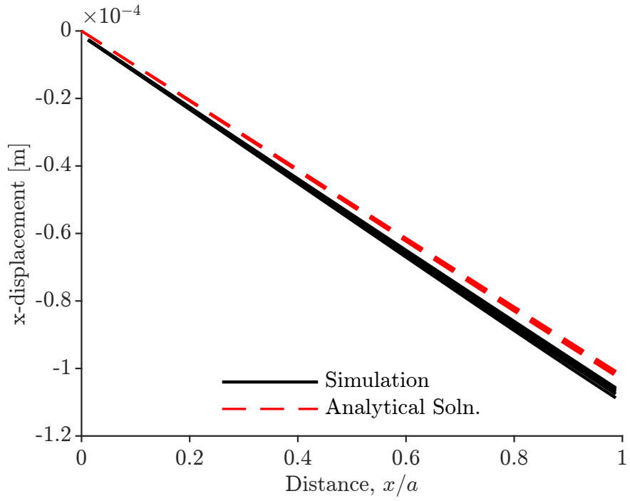
Figure 6: The MATLAB simulator results shown against the Mandel solution for various times.
