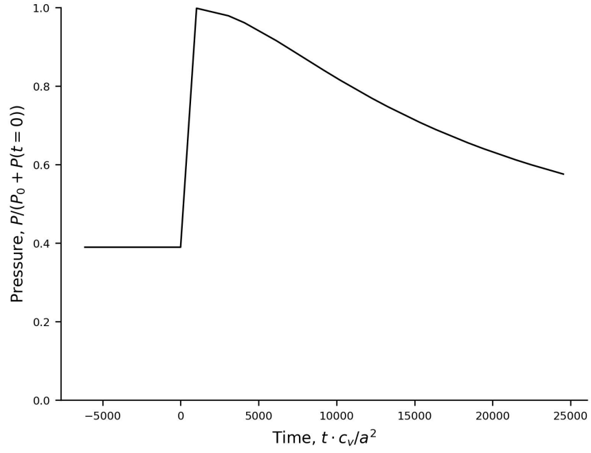
Figure 5: The Python simulator results. Note the Mandel-Cryer effect clearly visible at t = 0 . Additionally the jump in pressure matches the P_0 predicted for this problem.
