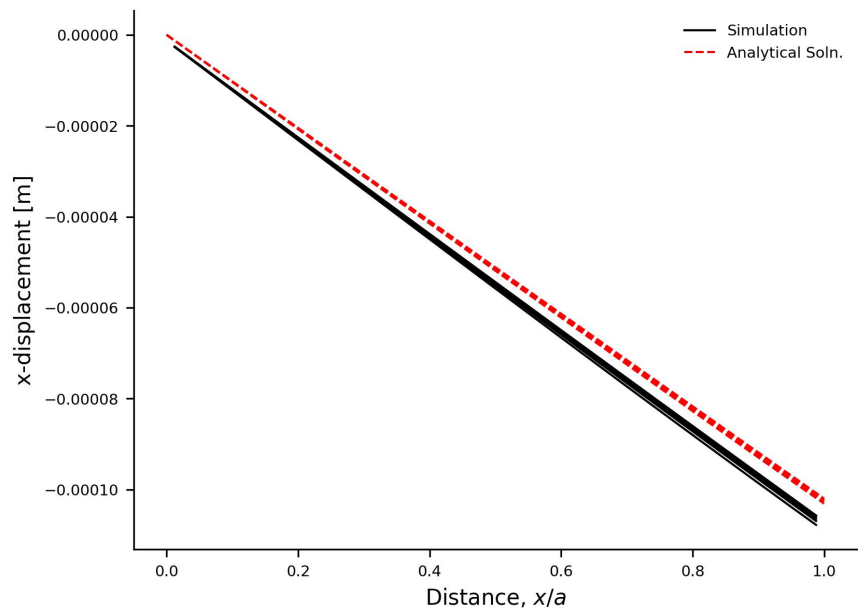
Figure 7: The Python simulator results shown against the Mandel solution for various times.
