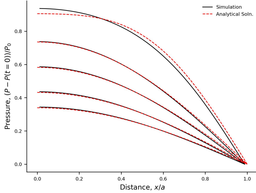
Figure 3: The Python simulator results shown against the Mandel solution for various times. Note that the simulator artificially sets the right-hand boundary to zero pressure using wells in the right-most cell, potentially resulting in slight numerical error. The solutions for the simulator are plotted for a height of 3a/2 .
