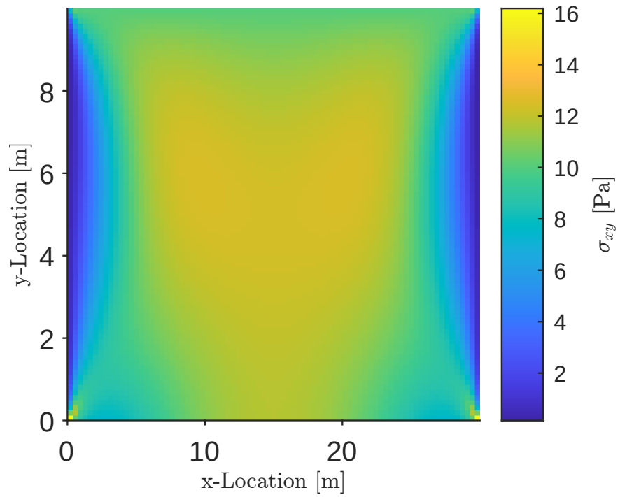
Figure 9: Shear stress found in MATLAB for a horizontal stress of -10 Pa applied to the top edge.
