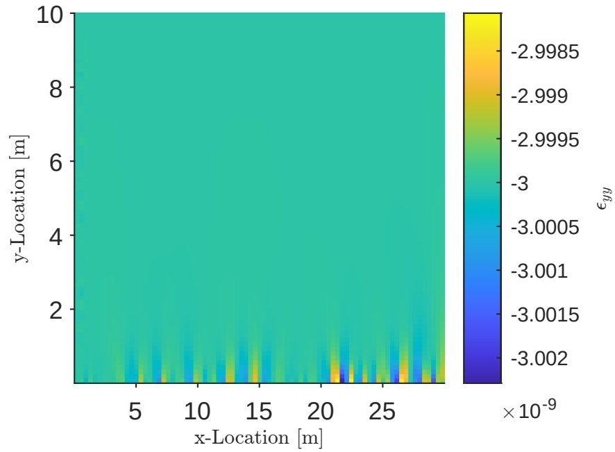
Figure 7: Vertical strain found in MATLAB for a horizontal stress of 10 Pa applied to the right edge.
