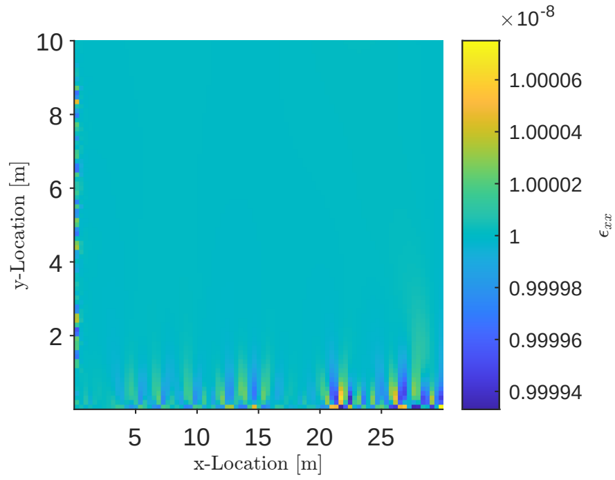
Figure 6: Horizontal strain found in MATLAB for a horizontal stress of 10 Pa applied to the right edge.
