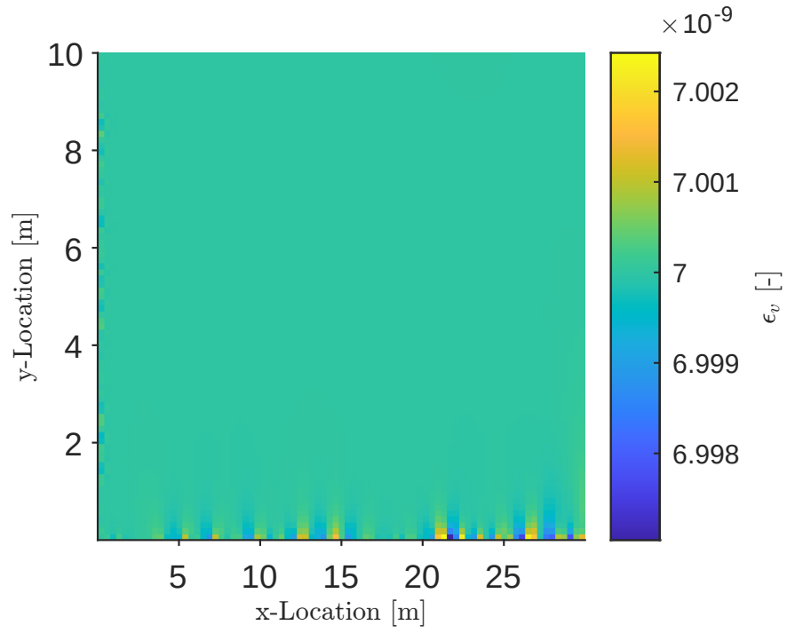
Figure 8: Volumetric strain found in MATLAB for a horizontal stress of 10 Pa applied to the right edge.
