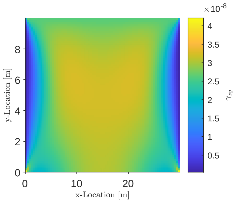
Figure 10: Engineering shear strain found in MATLAB for a horizontal stress of -10 Pa applied to the top edge.
