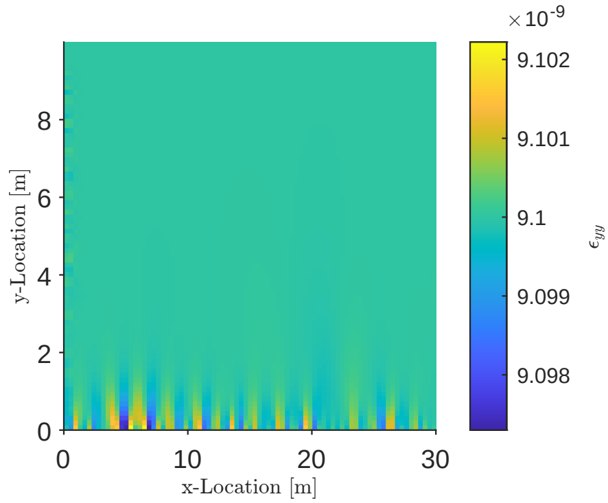
Figure 2: Vertical strain found in MATLAB for a vertical stress of 10 Pa applied to the top edge.
