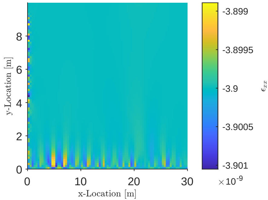
Figure 3: Horizontal strain found in MATLAB for a vertical stress of 10 Pa applied to the top edge.
