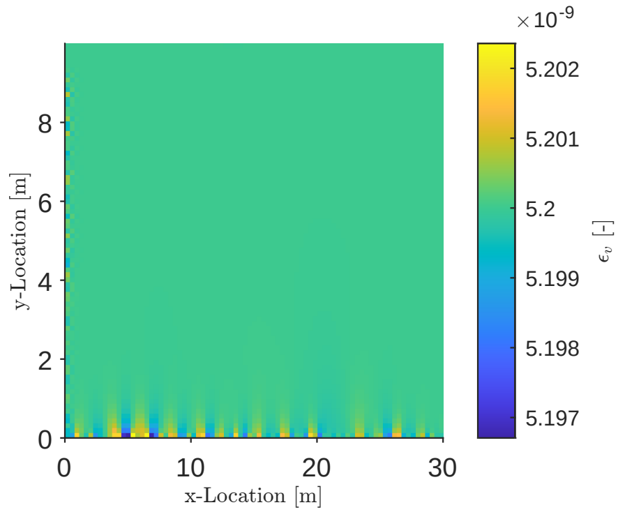
Figure 4: Volumetric strain found in MATLAB for a vertical stress of 10 Pa applied to the top edge.
