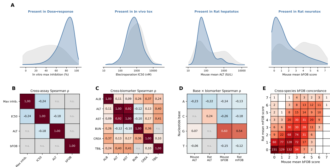
Figure 5: Selection bias, cross-assay and cross-biomarker correlations, base composition, and cross-species concordance. (A) Selection-bias KDEs showing biomarker distributions for compounds that do (blue) vs don't (grey) advance to the next pipeline stage. (B) Cross-assay Spearman \rho : pairwise correlations between per-compound metrics across pipeline stages (BH-corrected; n.s. = not significant). (C) Cross-biomarker Spearman \rho : correlations between mouse hepatotoxicity biomarkers (Bonferroni-corrected). (D) Nucleotide base × biomarker Spearman \rho : base composition vs toxicity biomarkers (BH-corrected). (E) Cross-species bFOB concordance: mouse bFOB vs rat mFOB score heatmap (integer-rounded); cell values are compound counts.
