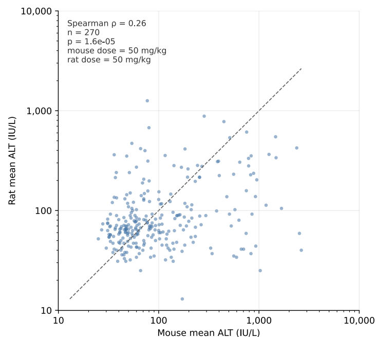
Figure 7: Cross-species hepatotoxicity concordance. Mean ALT per compound in mouse vs rat (log-log), with Spearman correlation shown.
