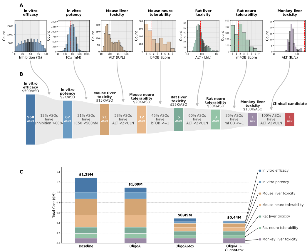
Figure 2: The ASO preclinical screening pipeline. (A) Distribution of measurements at each pipeline stage with pass/fail thresholds (red dashed lines); grey shading marks the failing region. (B) Attrition funnel showing the number of ASO candidates entering each stage, per-stage pass rates, and cumulative costs. Box heights are proportional to log(ASO count). (C) Cost savings from computational pre-screening: stacked bar chart comparing total pipeline costs by stage across four scenarios: baseline (no screening), OligoAI only (in vitro efficacy), OligoAI-tox only (ALT + bFOB), and all models combined.
