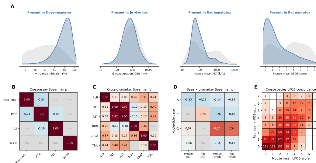
Figure 7: Selection bias, cross-assay and cross-biomarker correlations, base composition, and cross-species concordance. (A) Selection-bias KDEs showing biomarker distributions for compounds that do (blue) vs don't (grey) advance to the next pipeline stage. (B) Cross-assay Spearman \rho : pairwise correlations between per-compound metrics across pipeline stages (BH-corrected; n.s. = not significant). (C) Cross-biomarker Spearman \rho : correlations between mouse hepatotoxicity biomarkers (Bonferroni-corrected). (D) Nucleotide base \times biomarker Spearman \rho : base composition vs toxicity biomarkers (BH-corrected). (E) Cross-species bFOB concordance: mouse bFOB vs rat mFOB score heatmap (integer-rounded); cell values are compound counts.
