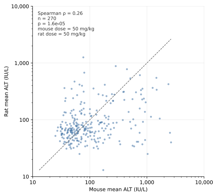
363 Figure 5: Cross-species hepatotoxicity concordance. Mean ALT per compound in mouse vs rat (log- 364 log), with Spearman correlation shown.
