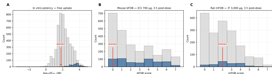
359 Figure 4: Clinical benchmark: ION582 (Zilganersen) in context of ASO Atlas 2.0 distributions. Grey 360 bars show all targets; blue bars highlight UBE3A-ATS -targeting ASOs; the red arrow marks ION582. 361 (A) IC 50 distribution under gymnosia/free-uptake conditions. (B) Mouse bFOB score distribution 362 (ICV, 700 µg, 3 h post-dose). (C) Rat mFOB score distribution (IT, 3,000 µg, 3 h post-dose).
