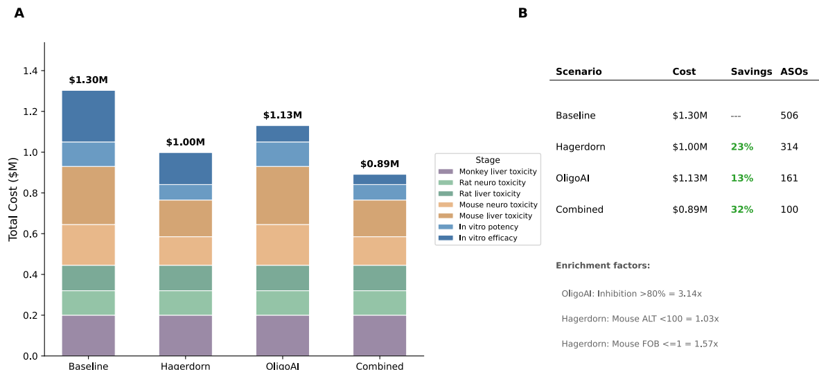
Figure 5: Cost savings from computational pre-screening. (A) Stacked bar chart comparing total pipeline costs by stage across four scenarios: baseline (no screening), Hagerdorn classifiers only (ALT + FOB), OligoAI only (in vitro efficacy), and all models combined. (B) Summary table of costs, savings, and enrichment factors.
