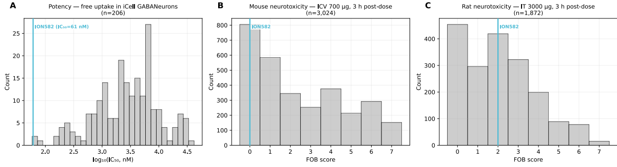
Figure 3: Benchmarking ION582 (zilganersen) against OligoStack distributions. (A) IC 50 distribution in iCell GABANeurons under free uptake conditions with ION582 marked. (B) Mouse FOB score distribution (ICV, 700 \mu\text{g} , 3 h post-dose). (C) Rat FOB score distribution (IT, 3000 \mu\text{g} , 3 h post-dose).
