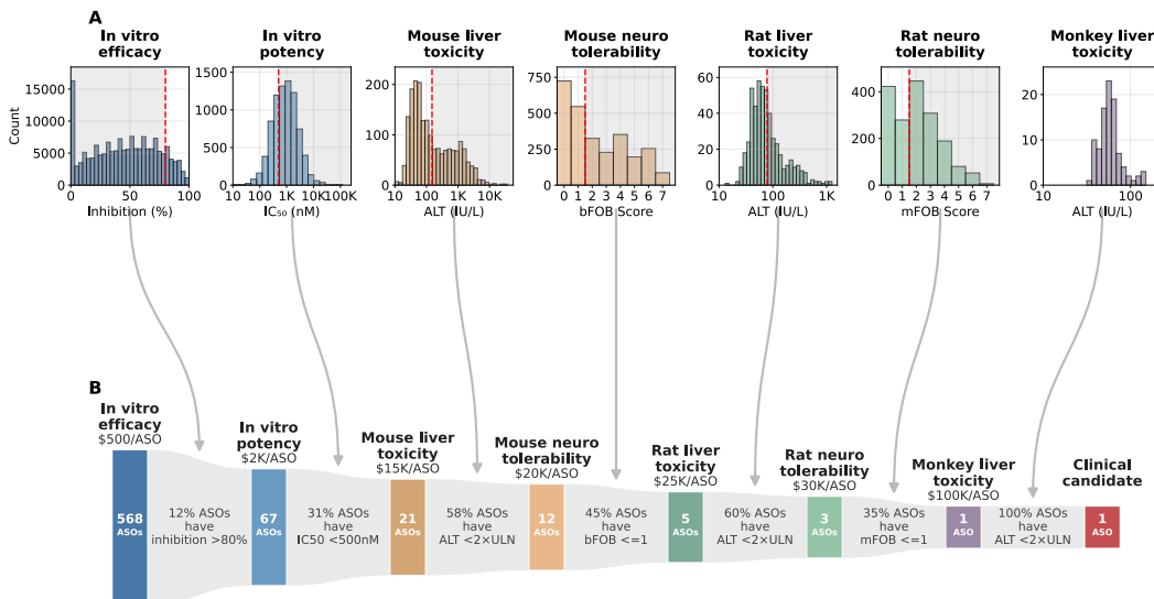
Figure 2: The ASO preclinical screening pipeline. (A) Distribution of measurements at each pipeline stage with pass/fail thresholds (red dashed lines); grey shading marks the failing region. (B) Attrition funnel showing the number of ASO candidates entering each stage, per-stage pass rates, and cumulative costs. Box heights are proportional to log(ASO count).
