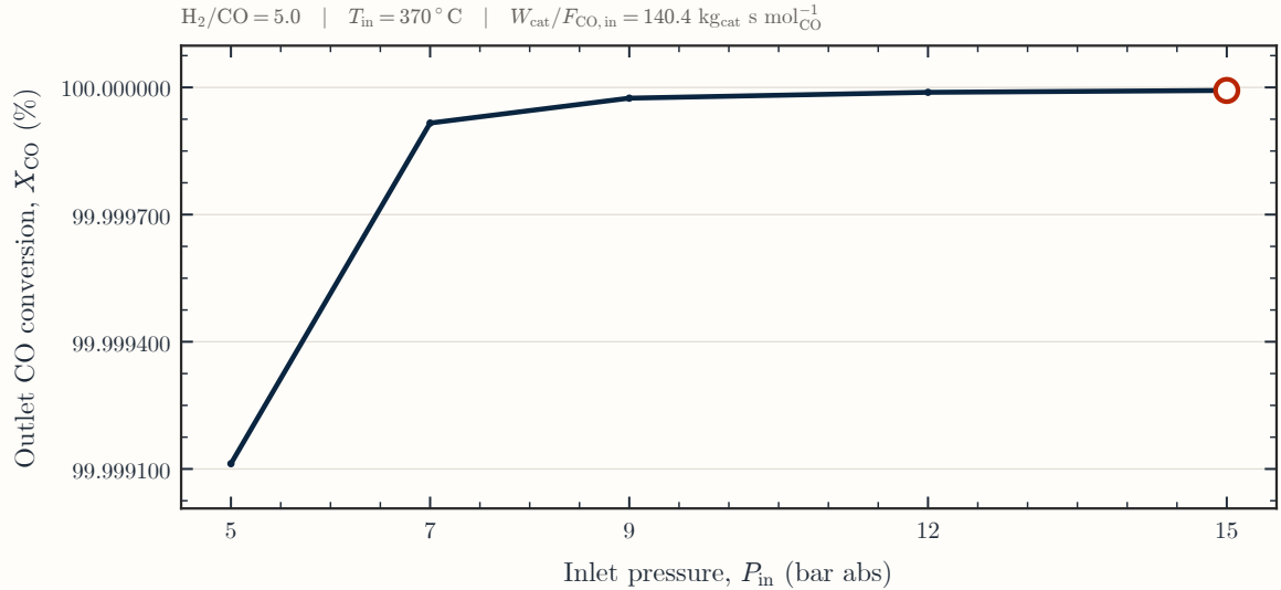
(c) Inlet pressure
