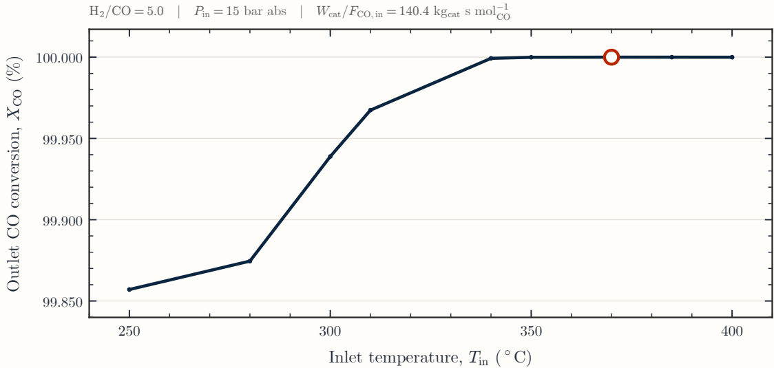
(b) Inlet temperature
