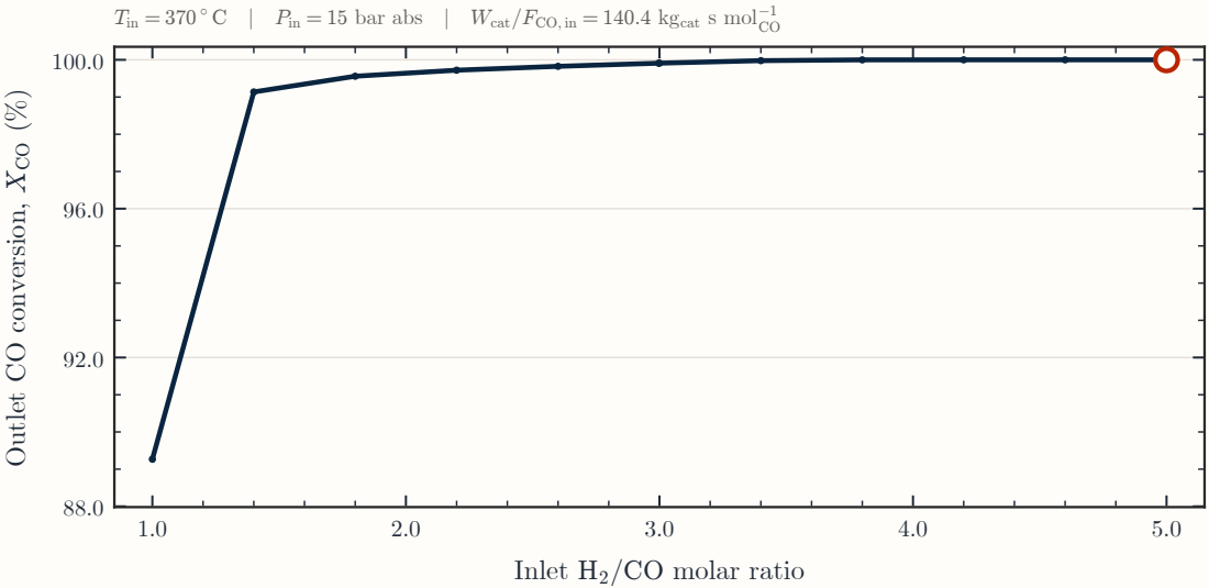
(a) \text{H}_2/\text{CO} feed ratio
