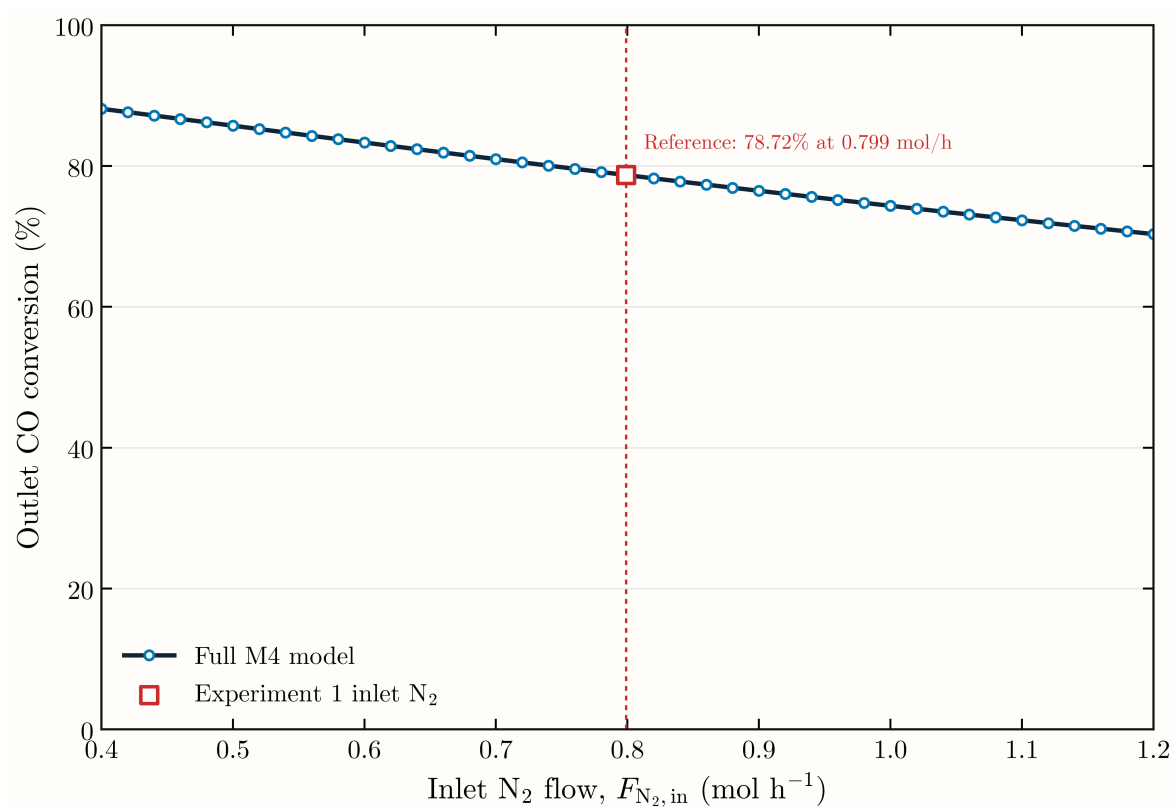
Figure 8. Full M4 predicted outlet CO conversion as inlet N 2 flow varies from 0.4 to 1.2 mol/h, with CO = 0.320 mol/h and H 2 = 0.959 mol/h fixed. The reference point at N 2 = 0.799 mol/h gives 78.72% conversion. Conditions are 350 °C, 1 bar absolute, and 3.12 g catalyst, isothermal and constant-pressure.
