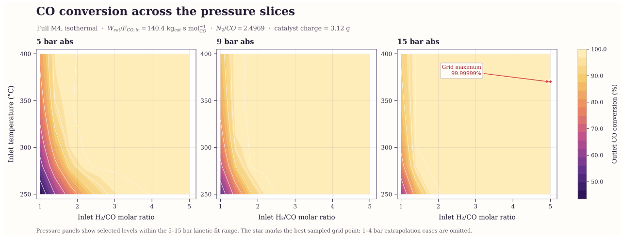
Figure 9. Pressure slices of predicted outlet CO conversion from the four-factor grid. Space time is fixed at 140.4 \text{ kg}_{\text{cat}} \text{ s mol}_{\text{CO}}^{-1} ; the star marks the best sampled point.
