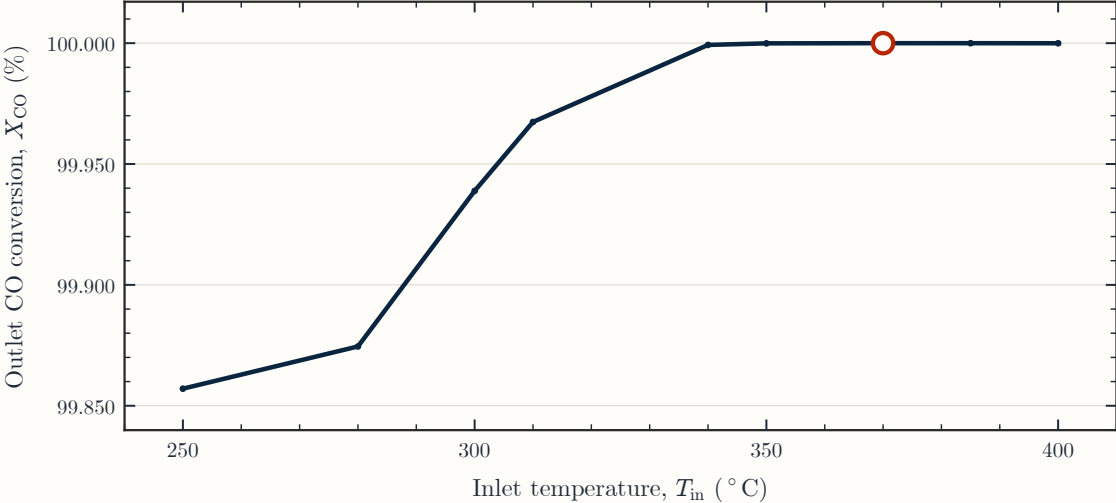
(b) Inlet temperature
