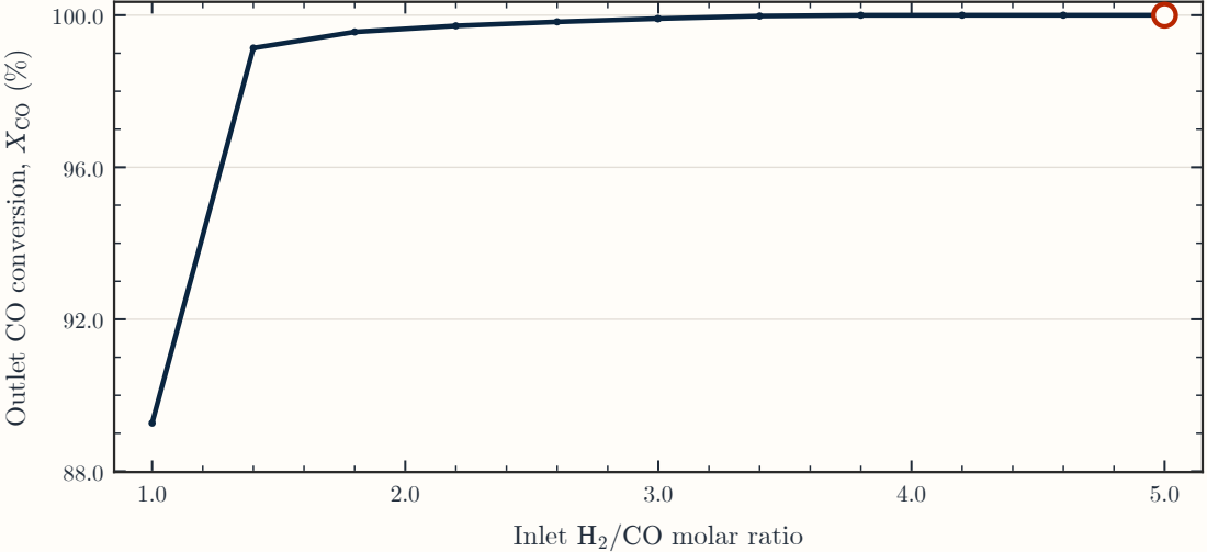
(a) \text{H}_2/\text{CO} feed ratio
