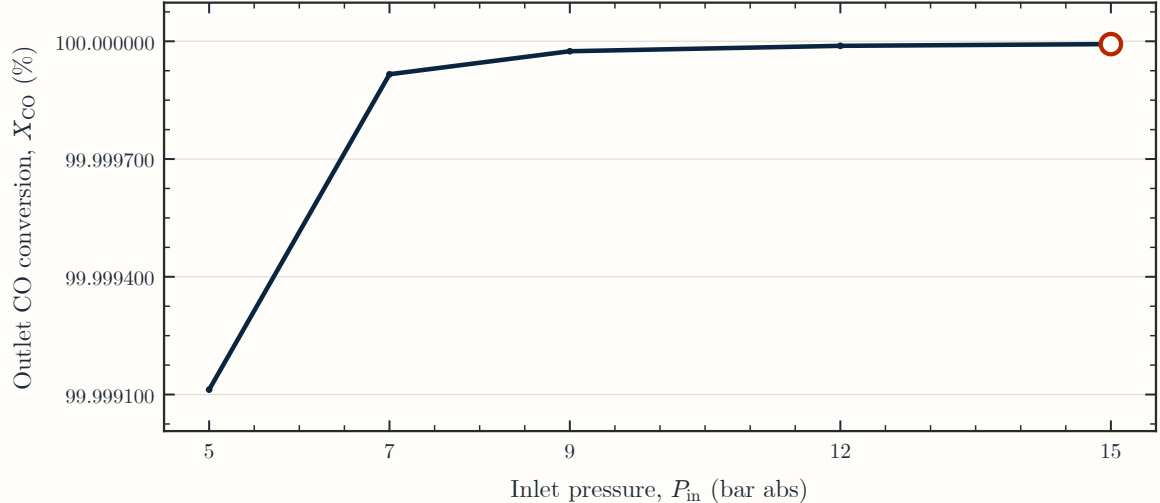
(c) Inlet pressure
