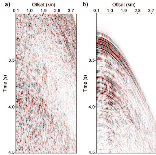
Figure 13.2: 3D SRME Example (Continued)
