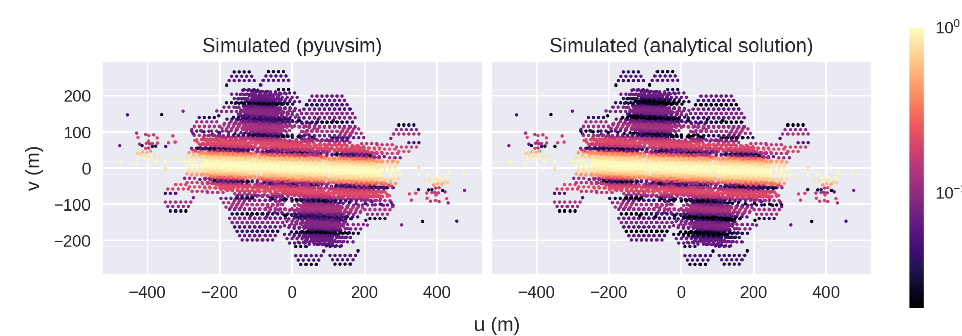
Figure 2. Comparison between the pyvusim simulation and the analytical Fourier model from Eq. 3 for the reference RFI event.
