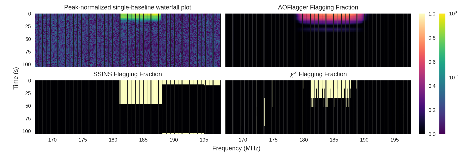
Figure 4. Top left: peak-normalized single-baseline waterfall plot for our reference observation. Top right: AOFlagger flagging fraction, calculated by averaging the output AOFlagger flag array along the baseline axis. Bottom left: SSINS flagging fraction. Bottom right: \chi^2 flagging fraction.
