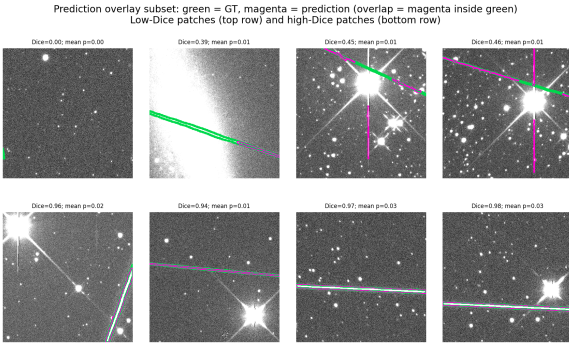
Figure 4: Representative test-patch predictions for the locked U-Net: ground truth in green, prediction in magenta, and overlap inside the green band.
