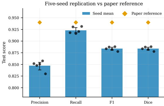
Figure 1: Five-seed replication performance for the locked U-Net compared with the Stoppa et al. reference. Recall is closely reproduced, while strict precision remains lower, motivating the boundary-scale error analysis.
