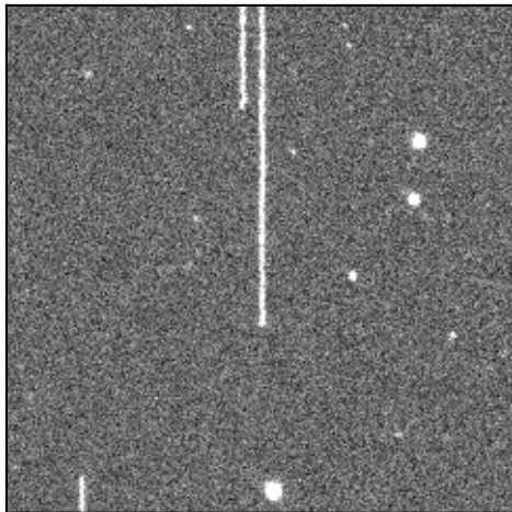
Audit crop
