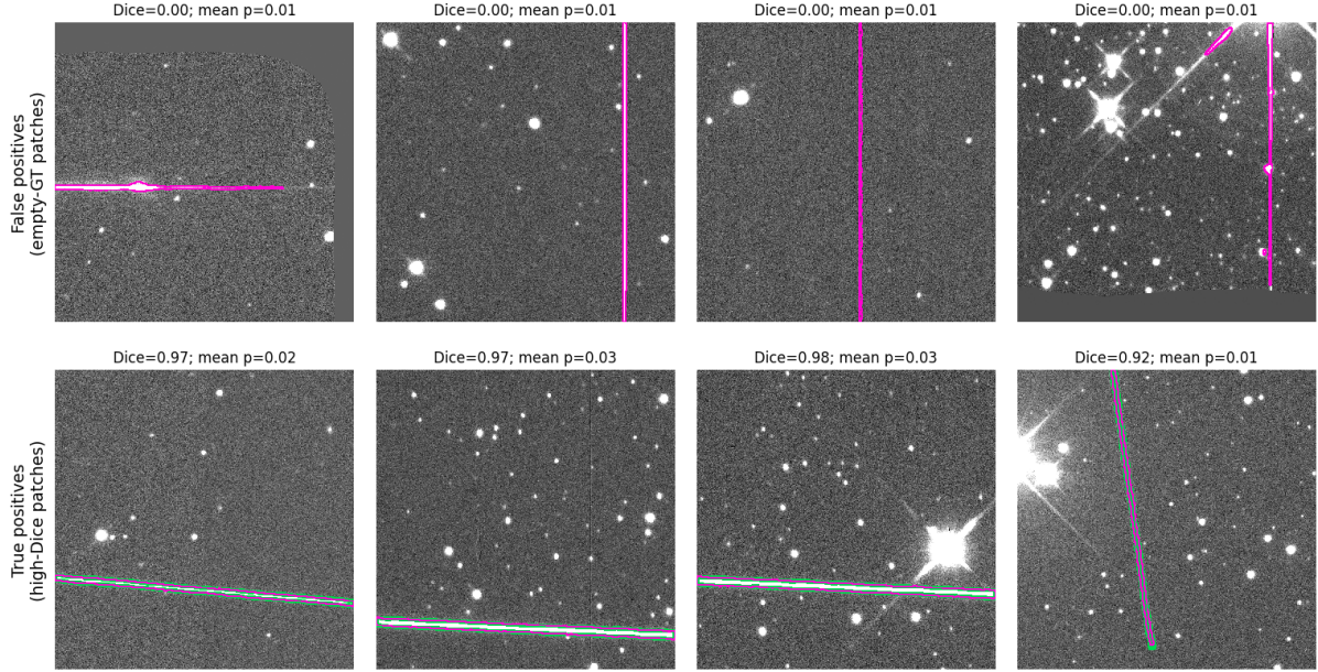
Figure B.6: False-positive and true-positive gallery for the locked winner, including bright-star diffraction-spike examples alongside high-Dice cases where bright stars are correctly ignored.
