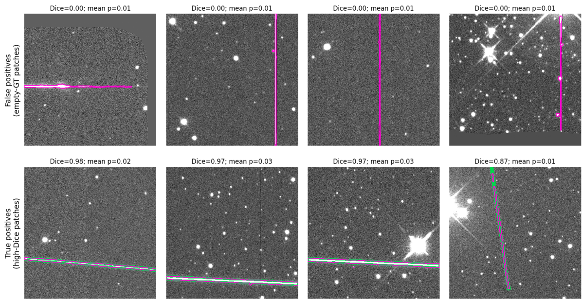
Figure B.7: The same eight patches for the attention-gated U-Net, in the order of Figure B.6, each with that model's own segmentation and Dice score.
