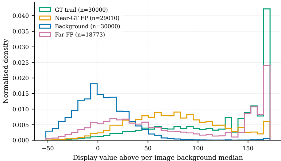
FP intensity rider: support-restricted U-Net pixels
