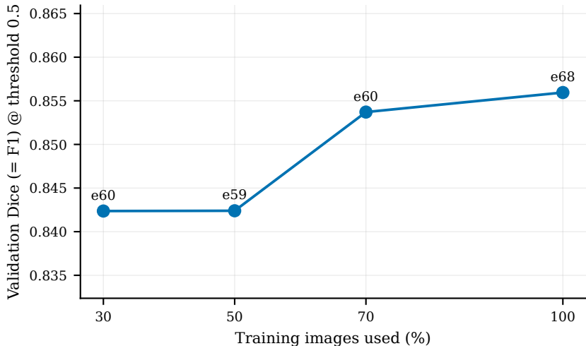
Data-efficiency curve (single seed 2804)
