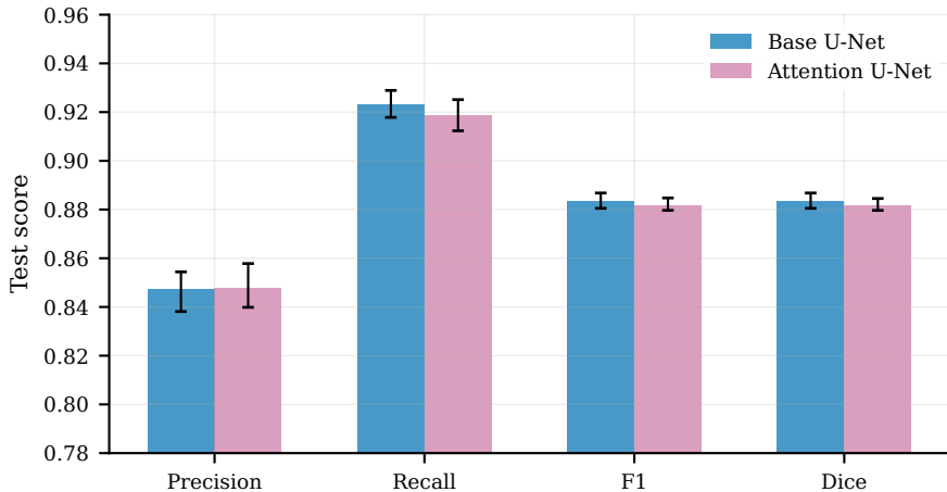
Base vs Attention U-Net
