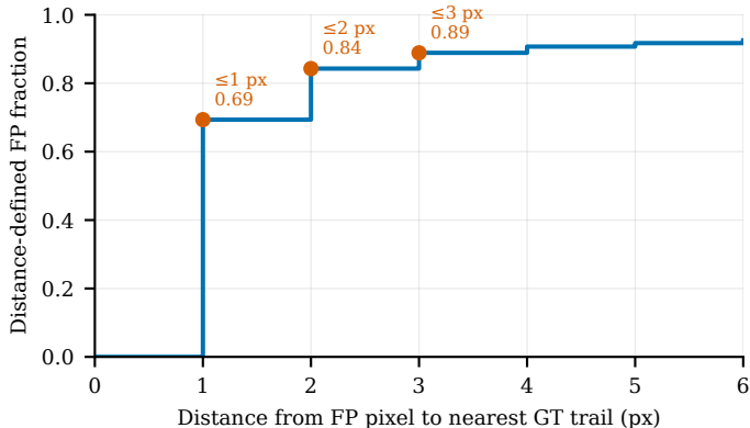
Cumulative distance-defined FP to nearest GT trail
