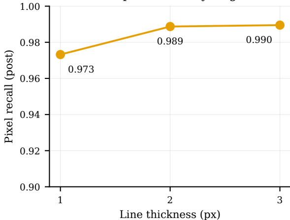
Completeness stays high
