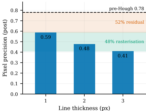
Strict-precision recovery
