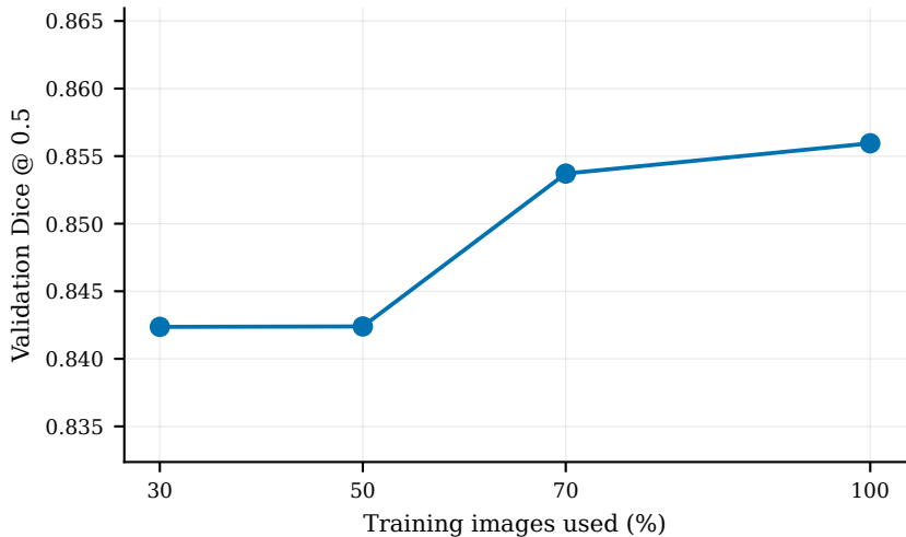
Data-efficiency curve
