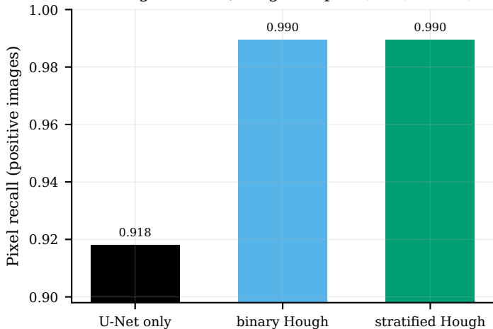
Stratified-Hough recall (Hough FP px: 2,725,702→2,785,274)
