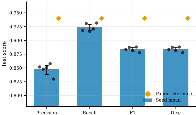
Five-seed replication vs paper reference
