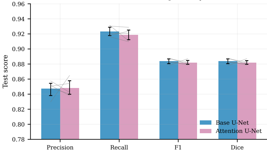
Base vs Attention U-Net, paired by seed
