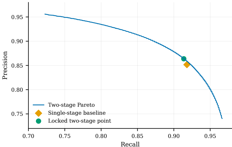
Classifier-gated operating characteristic (test-side, descriptive)
