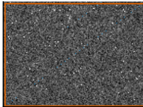
U-Net binary
