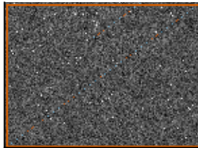
U-Net + Hough
