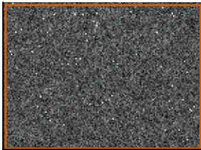
GT mask
