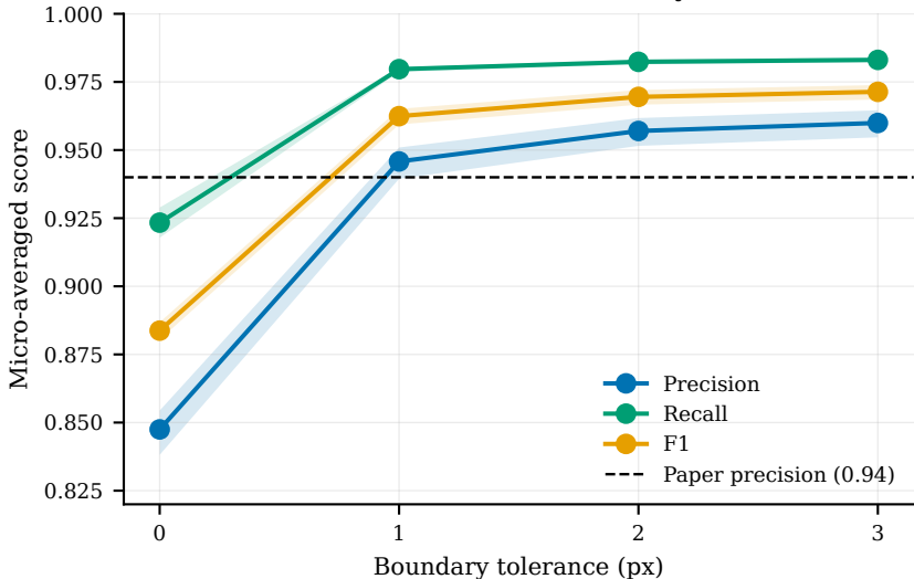
Precision/recall/F1 under boundary tolerance
