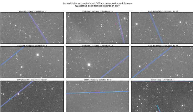
Figure 5: Cold-domain DECam examples: selected MeerLICHT-trained U-Net contours and Hough overlays on predeclared measured-streak frames. This is a qualitative transfer illustration, not a benchmark.
