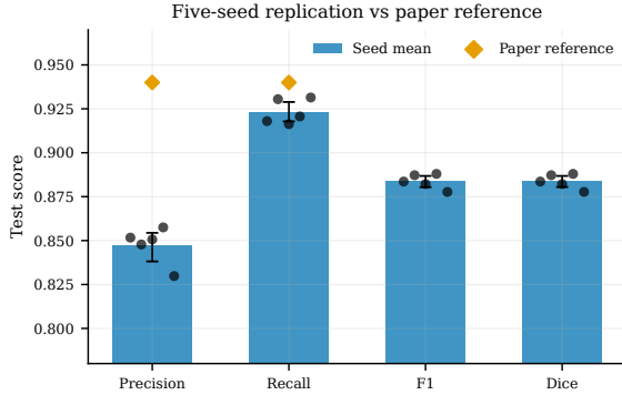
Figure 1: Five-seed replication performance for the selected U-Net compared with Stoppa et al. Paper-reference markers are shown only for the explicitly reported precision and recall values; recall is closely reproduced while pixel precision remains lower, motivating the boundary-near error analysis.
