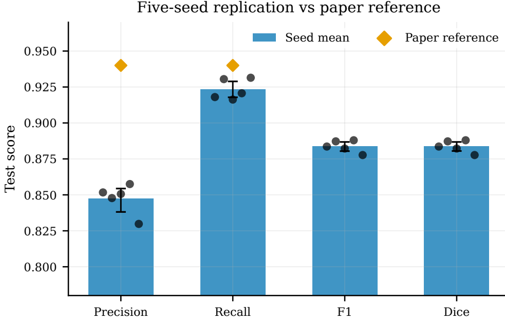
Figure 5.1: Five-seed replication summary for the locked validation-selected U-Net configuration. Paper-reference markers are shown only for the explicitly reported precision and recall values.
