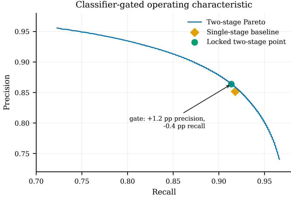
Figure 5.9: Two-stage operating-characteristic Pareto front over the classifier and U-Net thresholds; test-side and descriptive, not a validated improvement. The annotated point shifts precision +1.2 pp and recall -0.4 pp versus the locked baseline.
