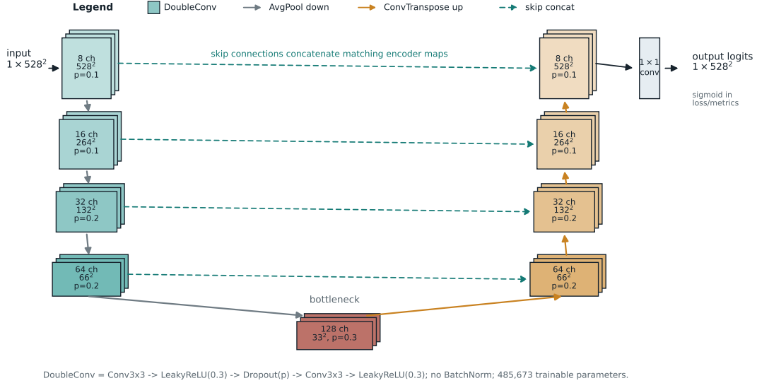
Figure 4.1: Architecture-faithful U-Net. Encoder widths 8 \rightarrow 16 \rightarrow 32 \rightarrow 64 with a 128-channel bottleneck, average-pooling downsampling, transposed-convolution up-sampling, and skip concatenation at each level. Each block is two 3 \times 3 convolutions with LeakyReLU(0.3) and in-block dropout.
