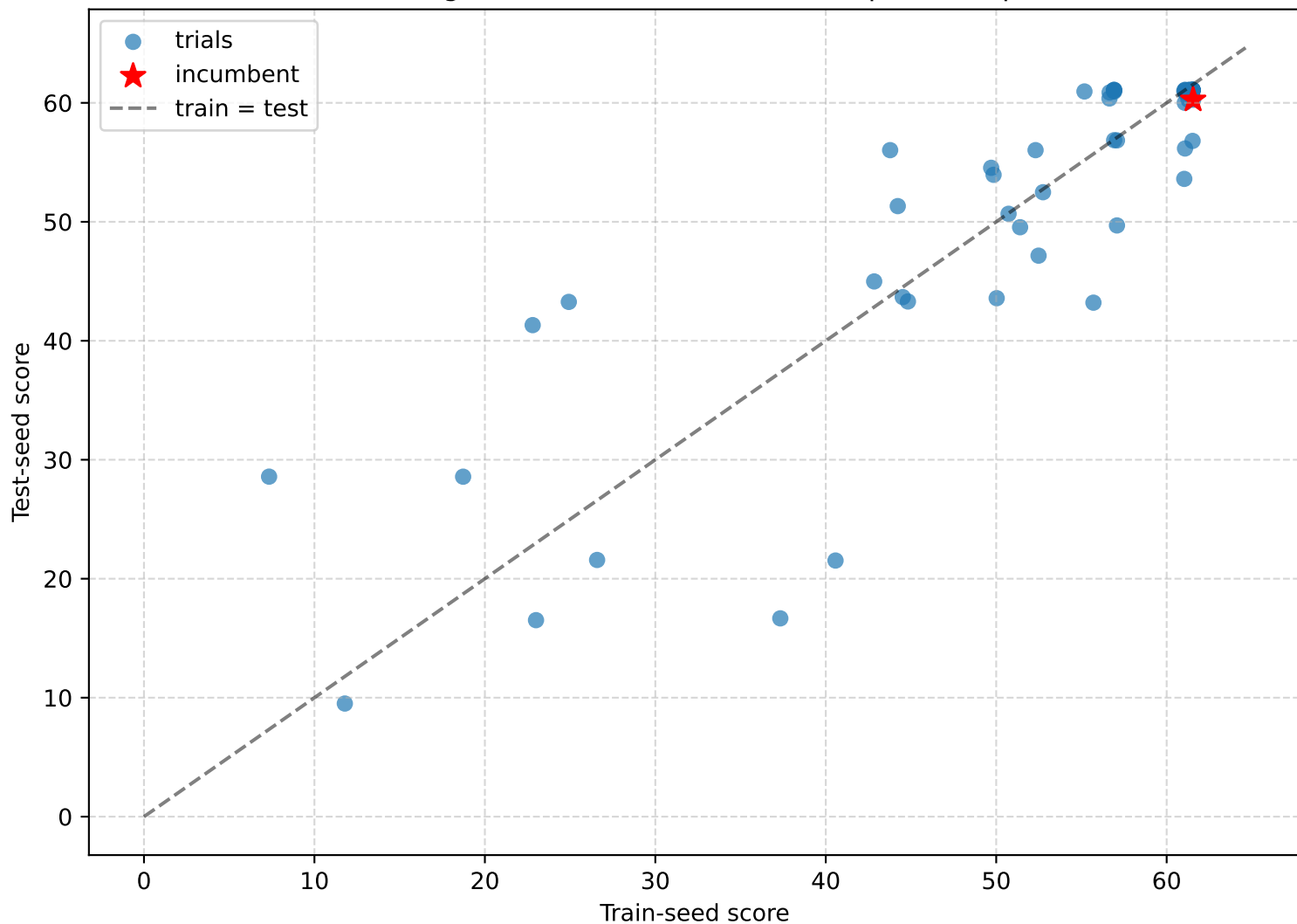
Level 1: HPO generalization across seeds (Spearman \rho = 0.81 )
