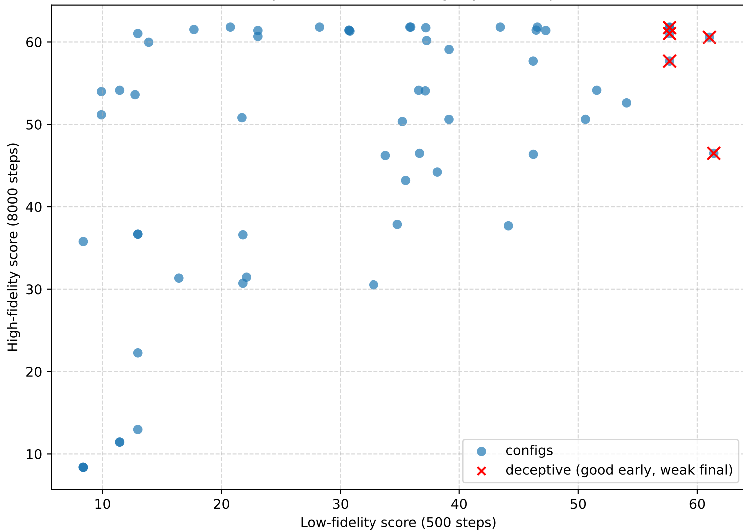
Level 2: early scores are deceiving (Spearman \rho = 0.45 )
