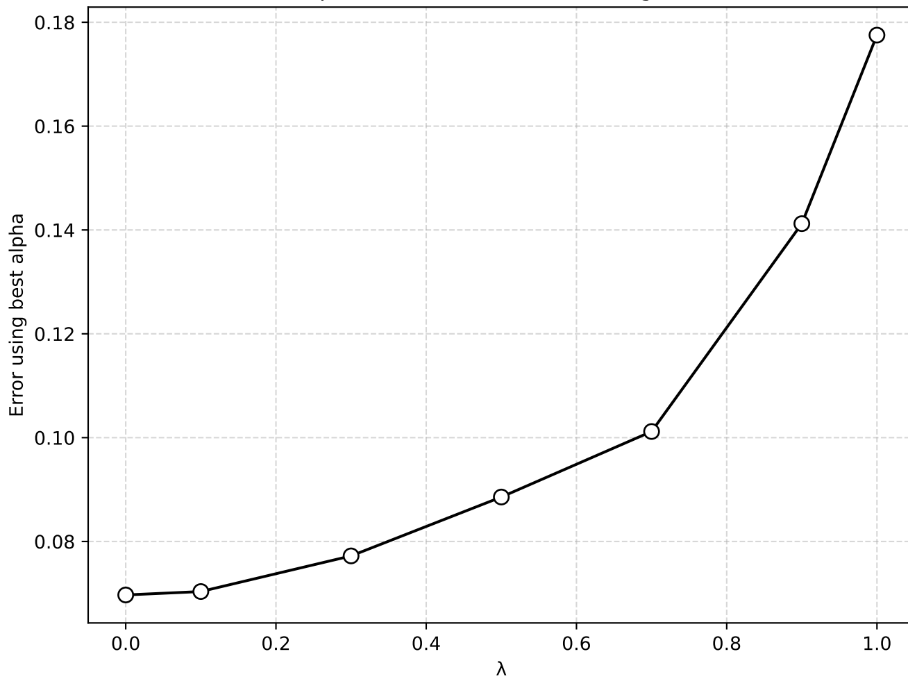
Reproduction Sutton (1988) - Figure 5
