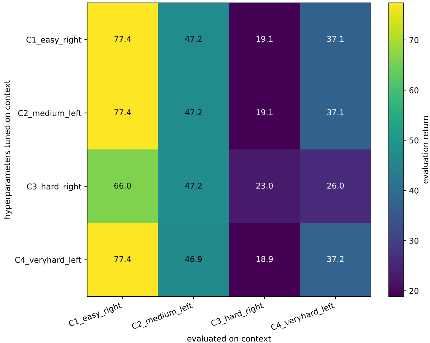
Level 3: hyperparameter transfer matrix
