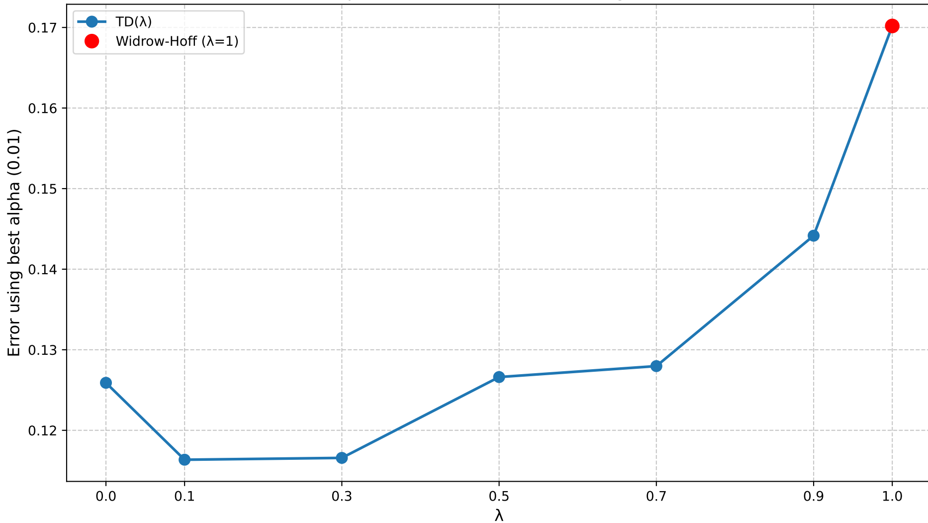
Reproduction Sutton (1988) - Figure 3
