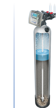
AirCat Iron and Hydrogen Sulfide Filter IPACG / IACG IPAG / IAG
