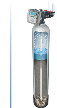
Air Iron Filter IMPFE / IMFE
