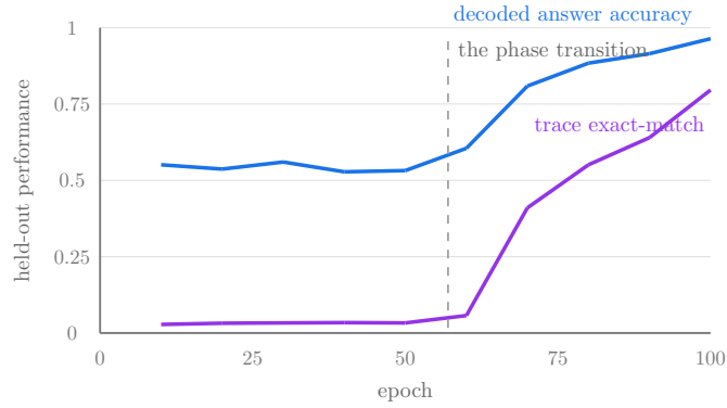
Figure 6: The grokking run: depth 2, 32k permuted graphs, zero regularization ( diameter_controlled , run 20260705_005620). Fifty flat epochs, then the circuit outcompetes memorization.
