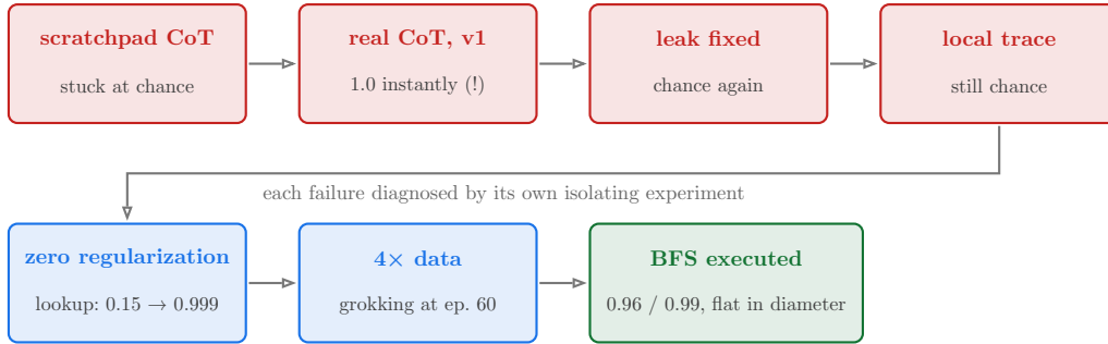
Figure 1: The route. Four configurations that failed for four different reasons, then two fixes that were about the optimizer and the data , not the architecture.
