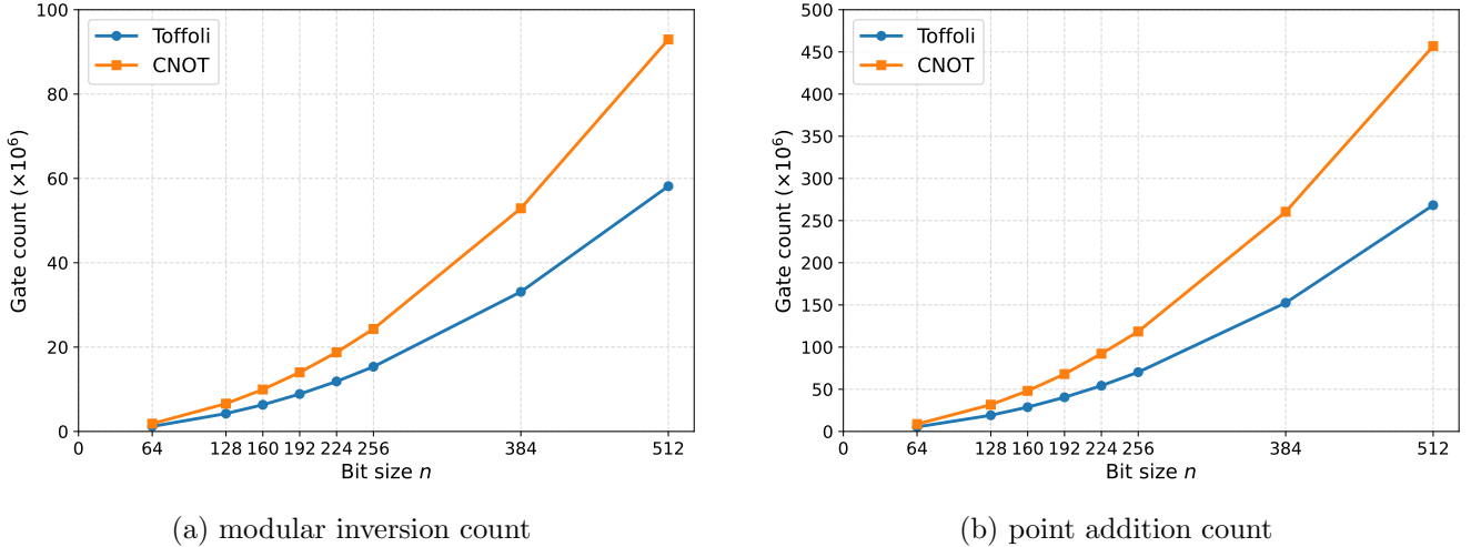
Figure 1: Toffoli gate count and CNOT gate count for modular inversion and point addition.
