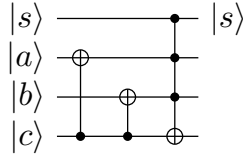
(a) Controlled MAJ cell.
