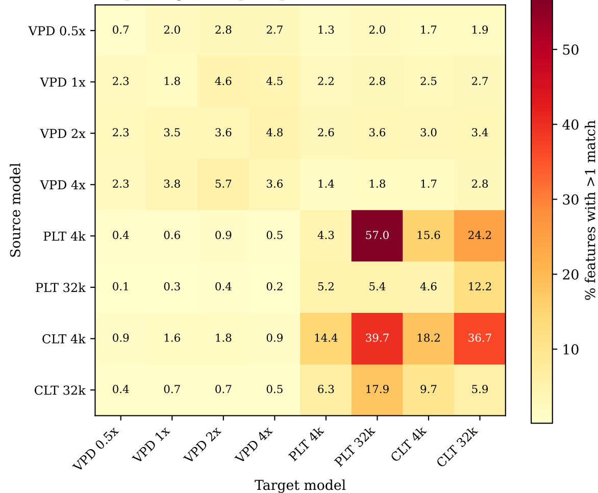
Feature splitting — output space (decoder / U) (cosine &gt; 0.5)
