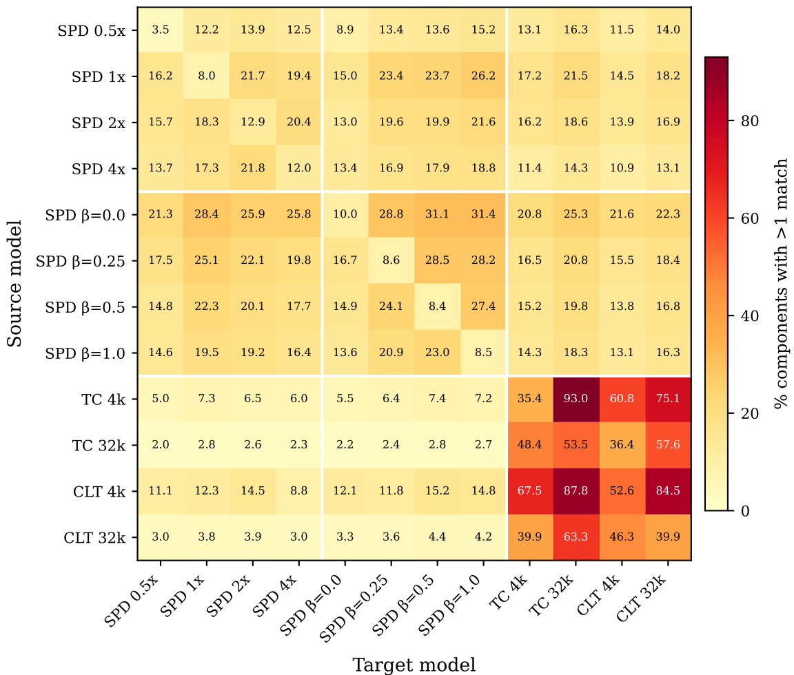
Cross-model component splitting (decoder / U, cosine &gt; 0.3)
