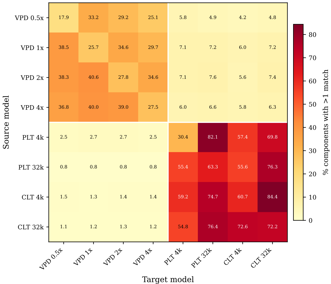
Cross-model component splitting (encoder / V, cosine &gt; 0.3)
