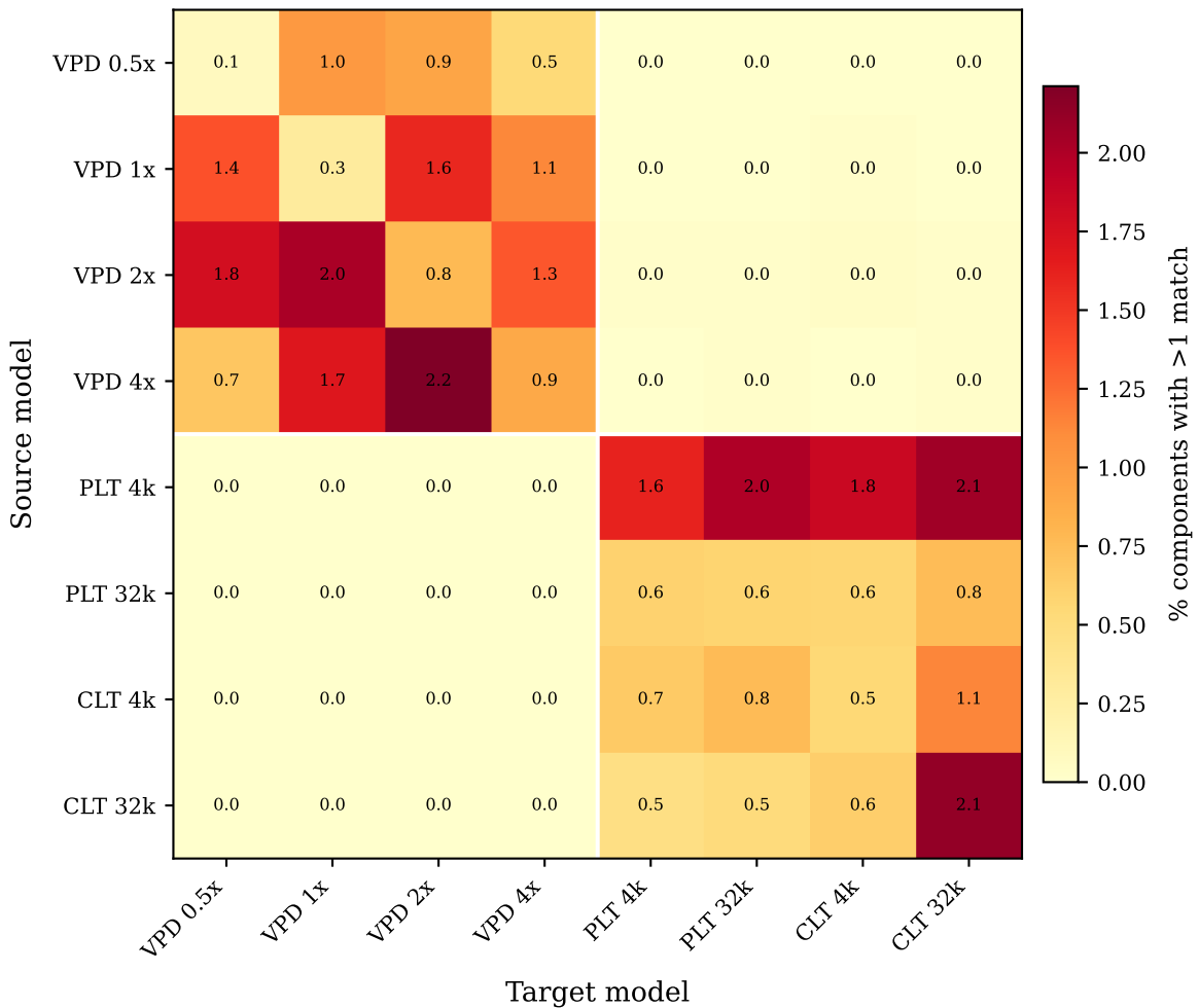
Cross-model component splitting (encoder / V, cosine &gt; 0.7)
