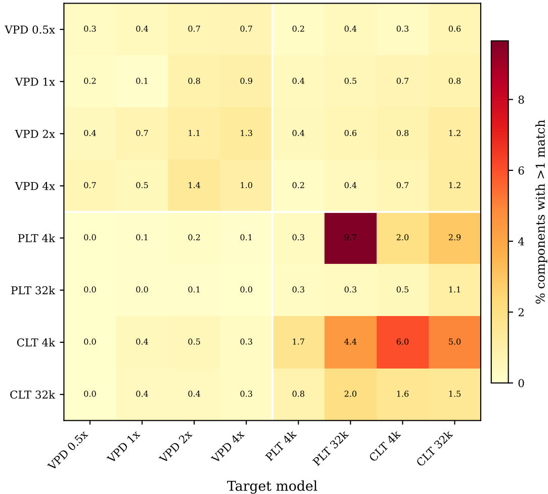
Cross-model component splitting (decoder / U, cosine &gt; 0.7)
