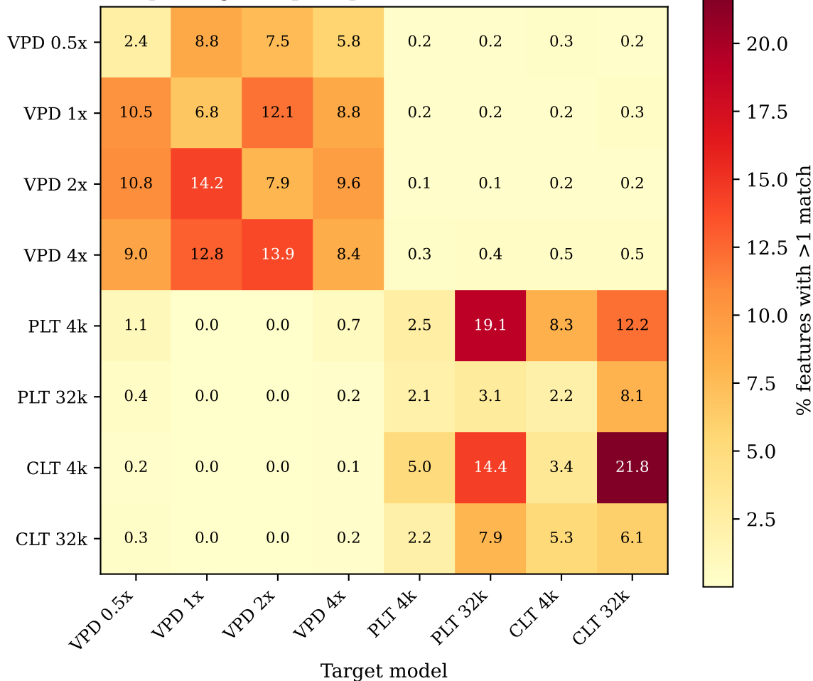
Feature feature splitting — input space (encoder / V) (cosine &gt; 0.5)
