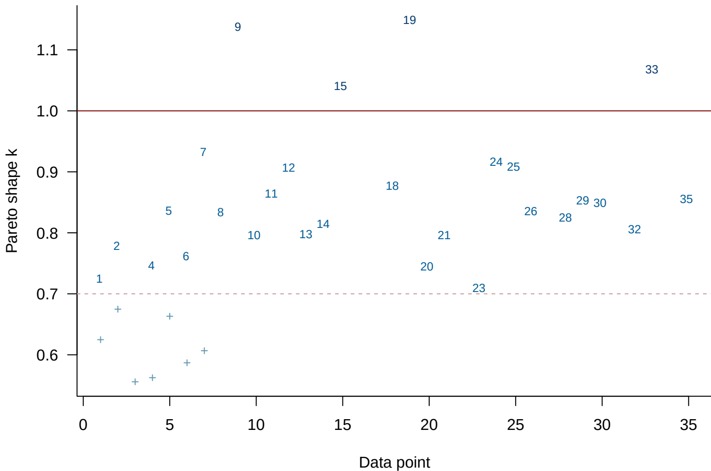
PSIS diagnostic plot
