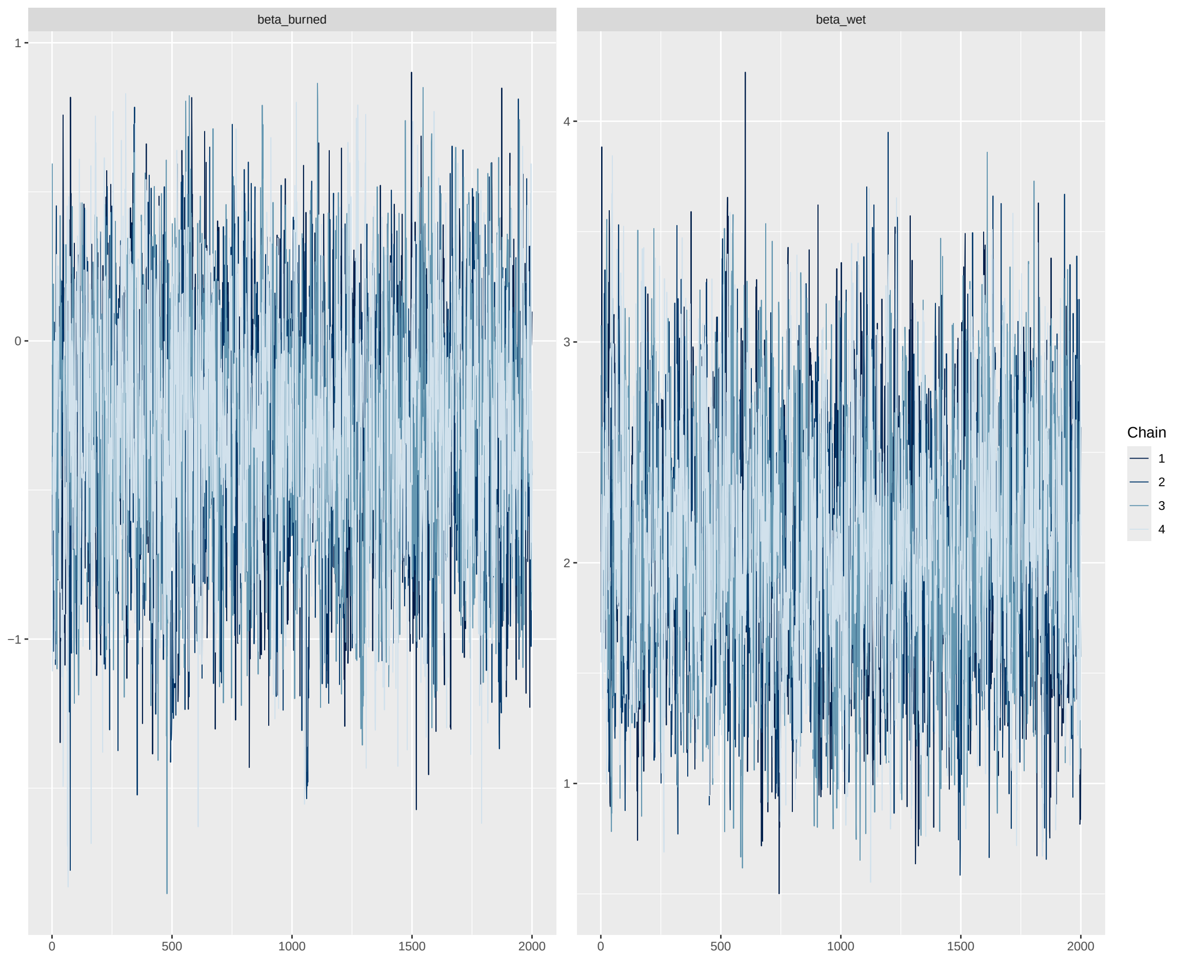
Trace Plots: Effects on Stream Quality
