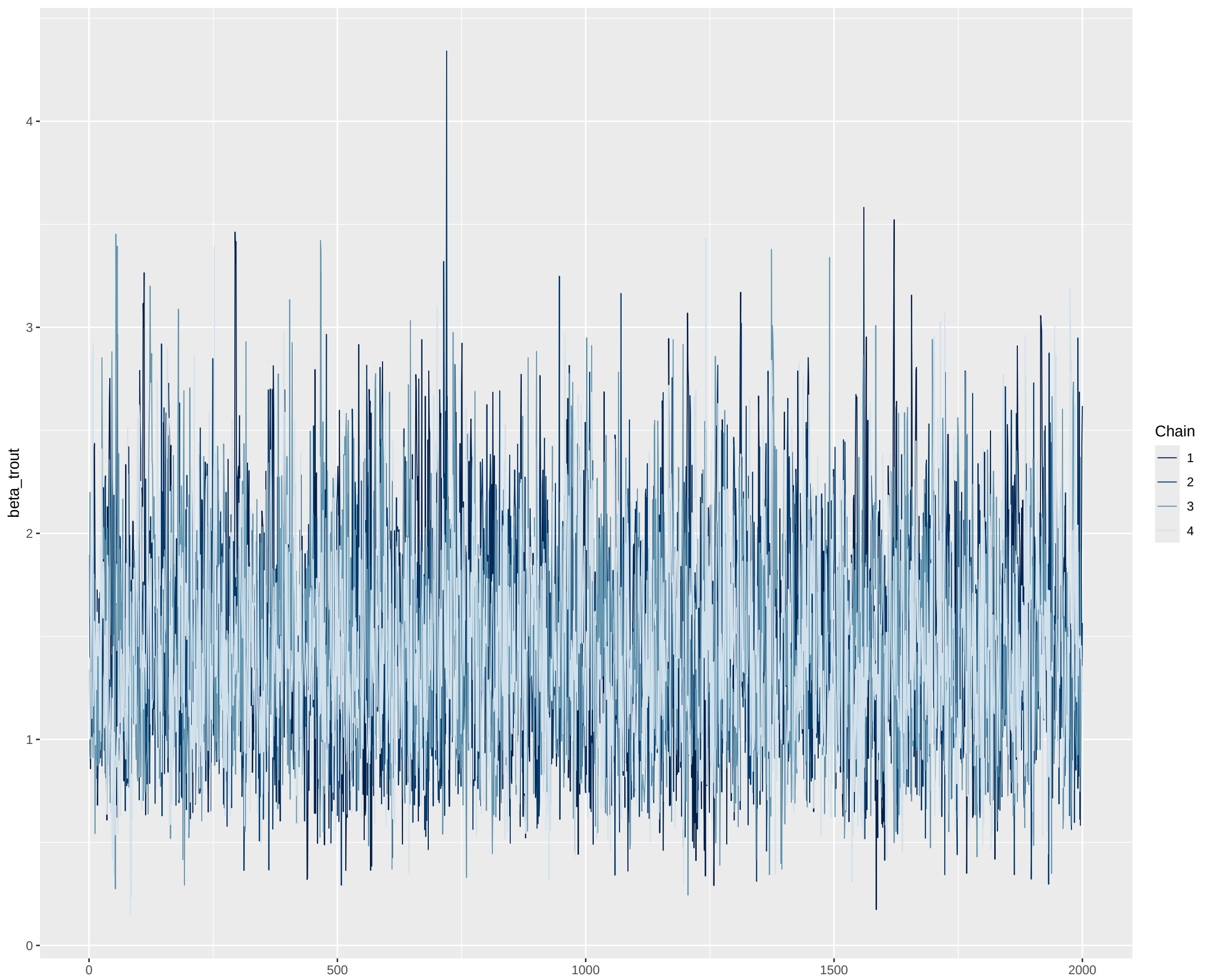
Trace Plots: Effect on Trout
