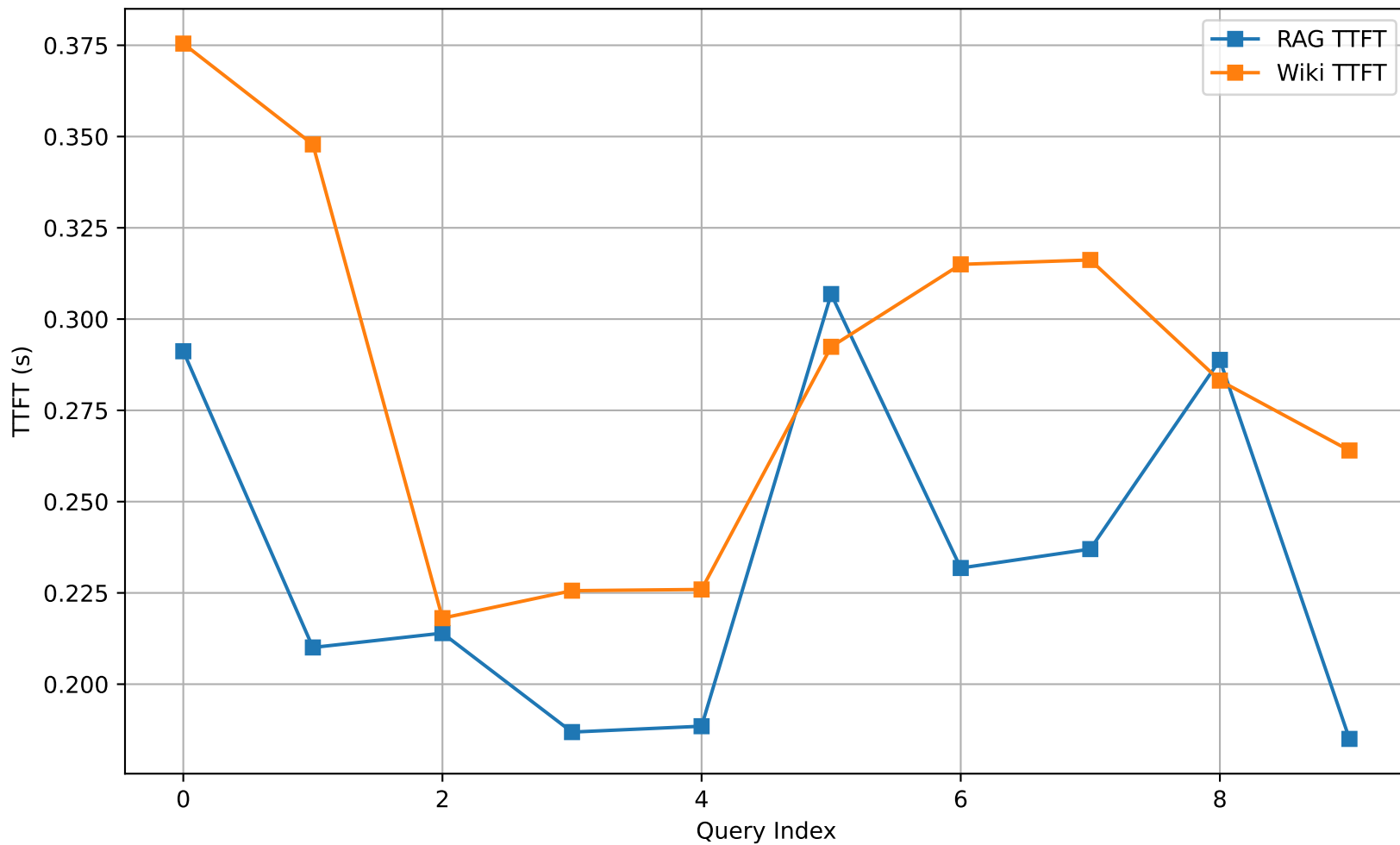
Time To First Token (TTFT)
